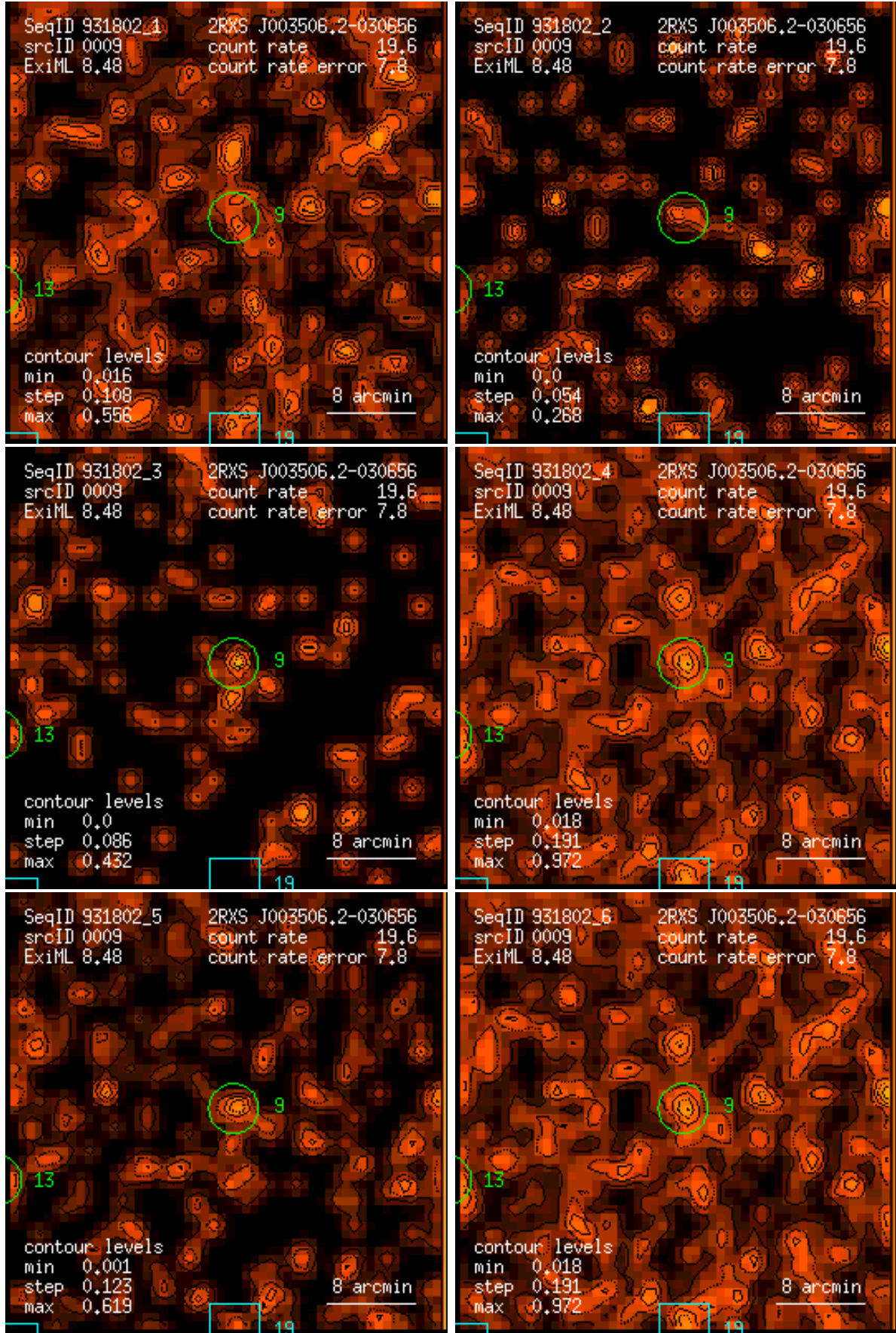
Figure 9: RASS 931802: detection 0009: band rate images, Gaussian filter: (1) PSPC channels 11 – 41, (2) 52 – 90, (3) 91 – 201, (4) 11 – 235, (5) 52 – 201, (6) 11 – 201. Broad band rates in counts/ks. Band rate contour levels in counts/ks/arcmin 2 .
