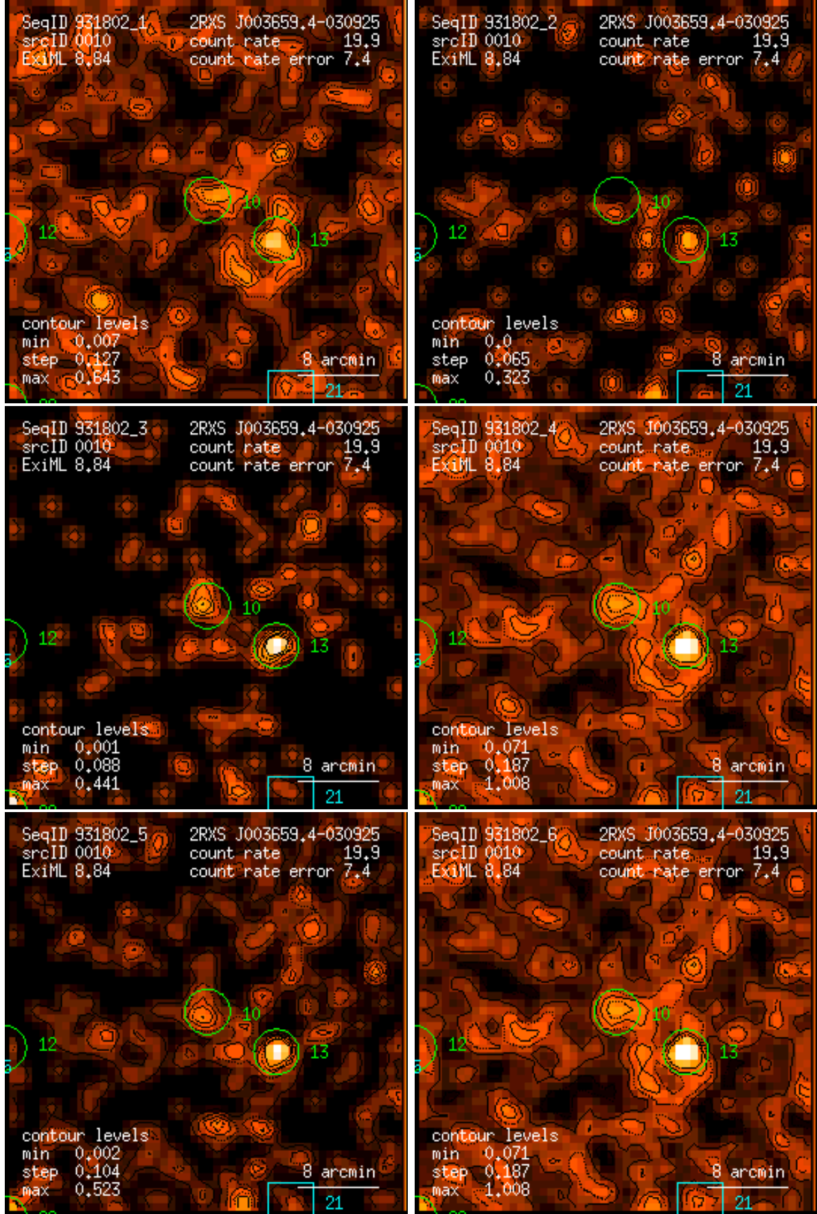
Figure 10: RASS 931802: detection 0010: band rate images, Gaussian filter: (1) PSPC channels 11 – 41, (2) 52 – 90, (3) 91 – 201, (4) 11 – 235, (5) 52 – 201, (6) 11 – 201. Broad band rates in counts/ks. Band rate contour levels in counts/ks/arcmin 2 .
