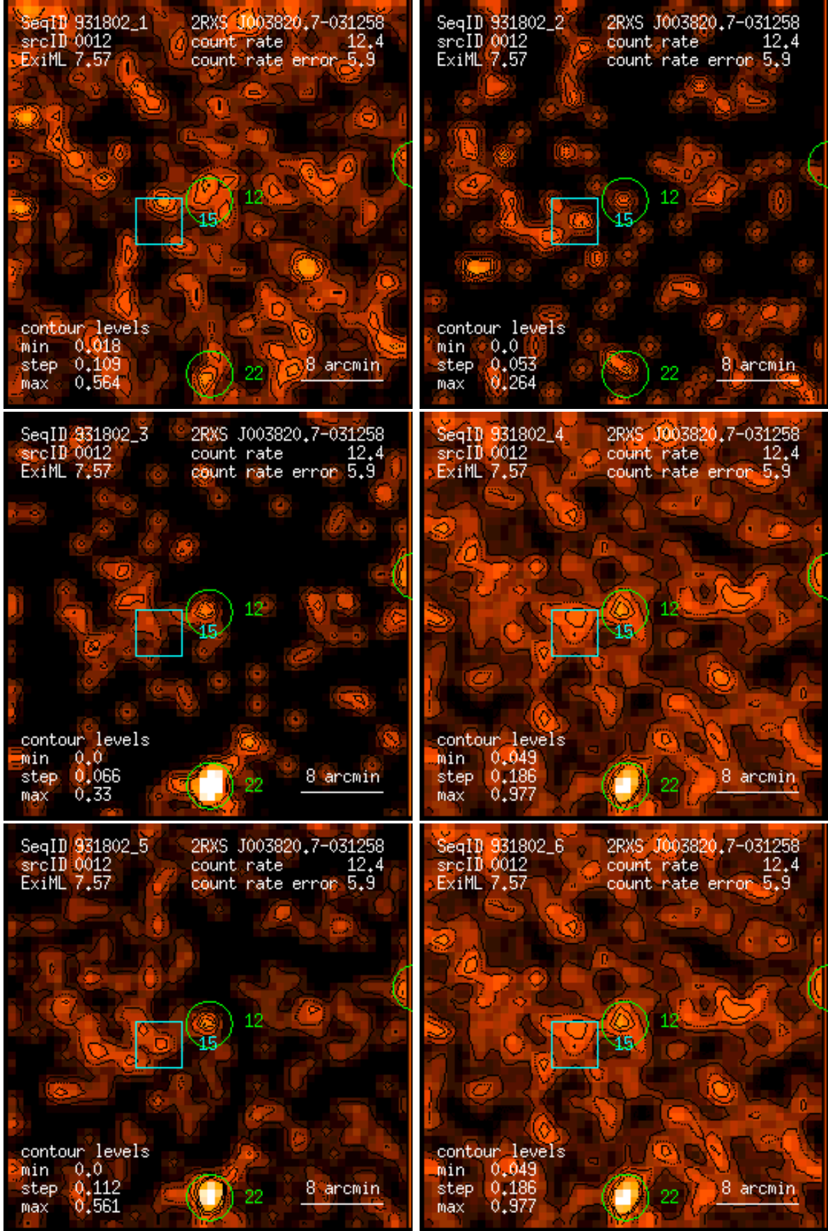
Figure 12: RASS 931802: detection 0012: band rate images, Gaussian filter: (1) PSPC channels 11 – 41, (2) 52 – 90, (3) 91 – 201, (4) 11 – 235, (5) 52 – 201, (6) 11 – 201. Broad band rates in counts/ks. Band rate contour levels in counts/ks/arcmin 2 .
