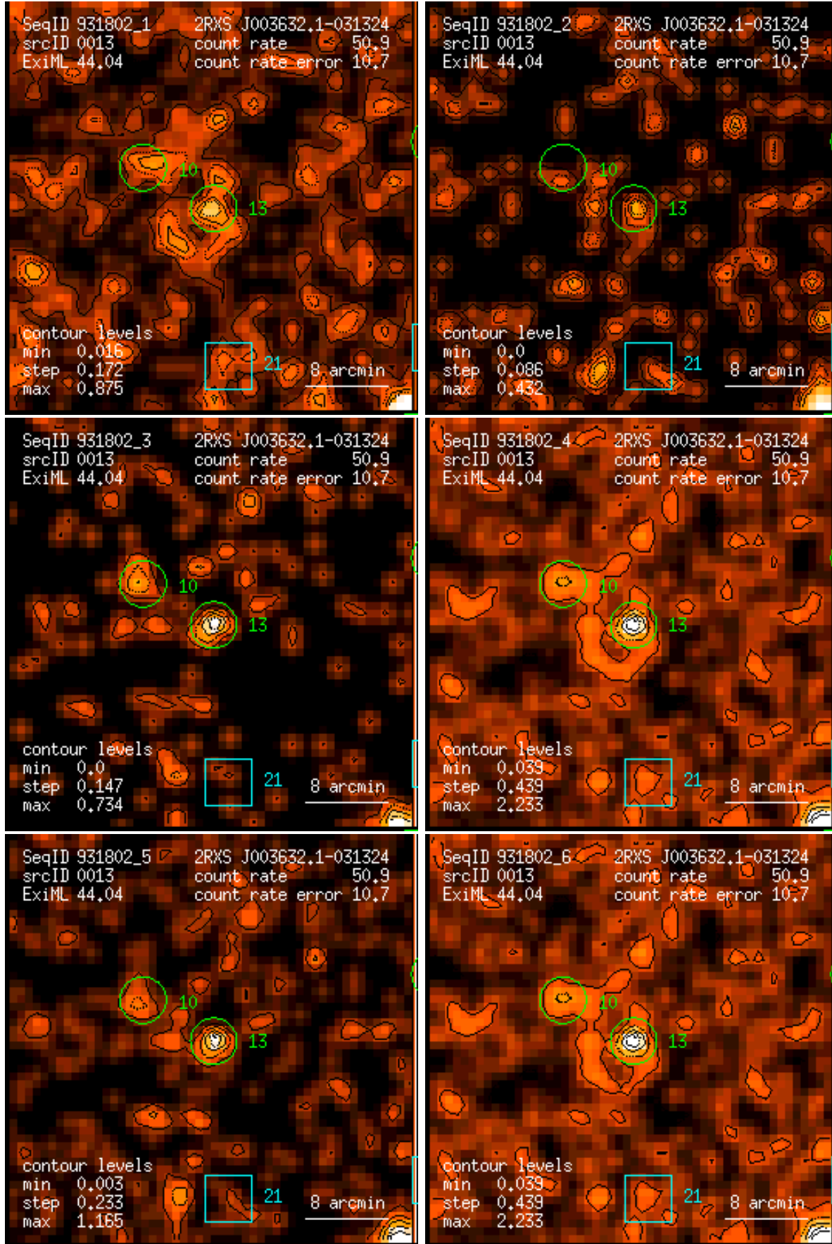
Figure 13: RASS 931802: detection 0013: band rate images, Gaussian filter: (1) PSPC channels 11 – 41, (2) 52 – 90, (3) 91 – 201, (4) 11 – 235, (5) 52 – 201, (6) 11 – 201. Broad band rates in counts/ks. Band rate contour levels in counts/ks/arcmin 2 .
