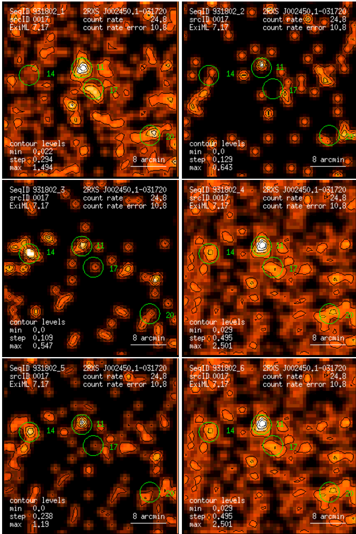
Figure 17: RASS 931802: detection 0017: band rate images, Gaussian filter: (1) PSPC channels 11 – 41, (2) 52 – 90, (3) 91 – 201, (4) 11 – 235, (5) 52 – 201, (6) 11 – 201. Broad band rates in counts/ks. Band rate contour levels in counts/ks/arcmin 2 .
