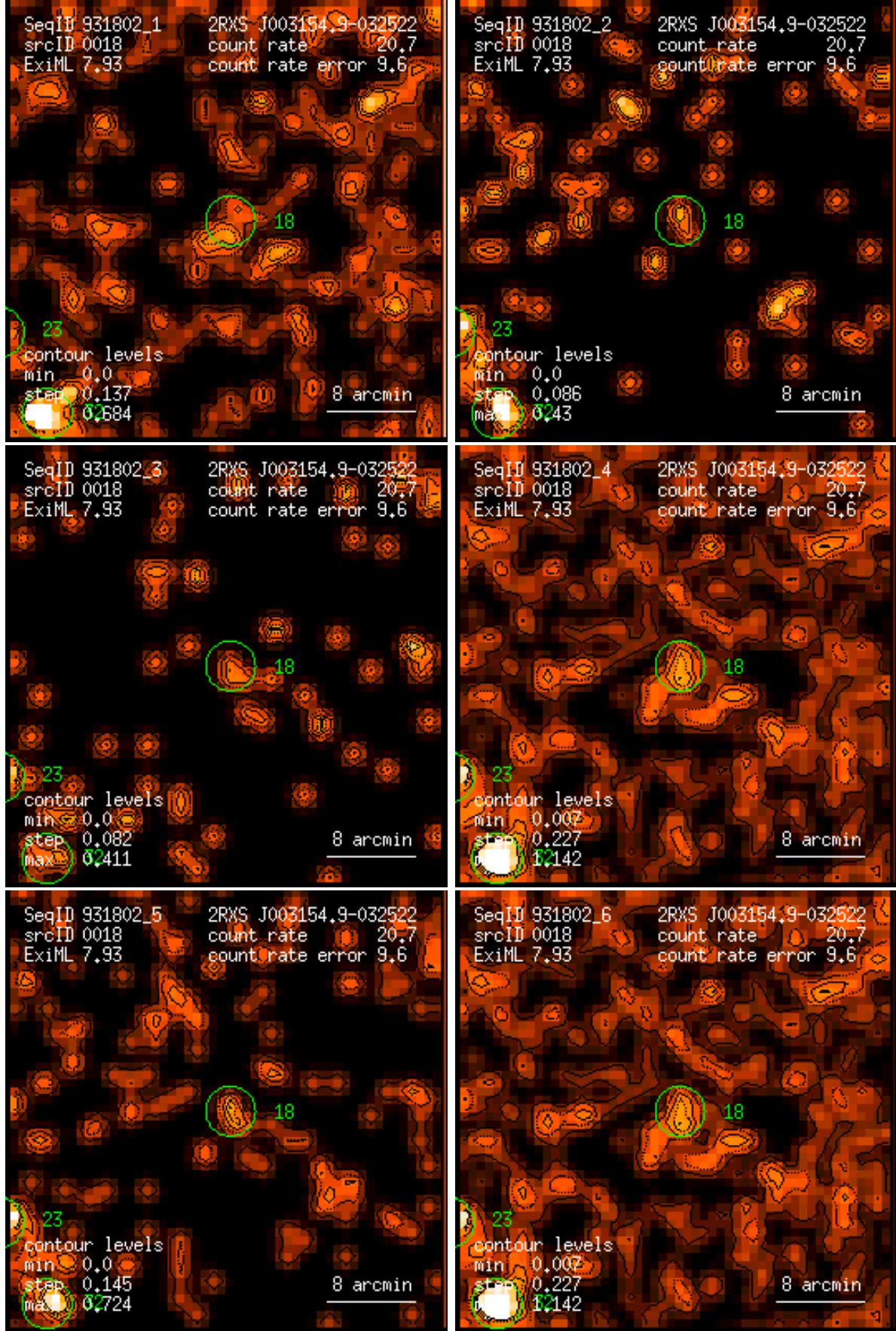
Figure 18: RASS 931802: detection 0018: band rate images, Gaussian filter: (1) PSPC channels 11 – 41, (2) 52 – 90, (3) 91 – 201, (4) 11 – 235, (5) 52 – 201, (6) 11 – 201. Broad band rates in counts/ks. Band rate contour levels in counts/ks/arcmin 2 .
