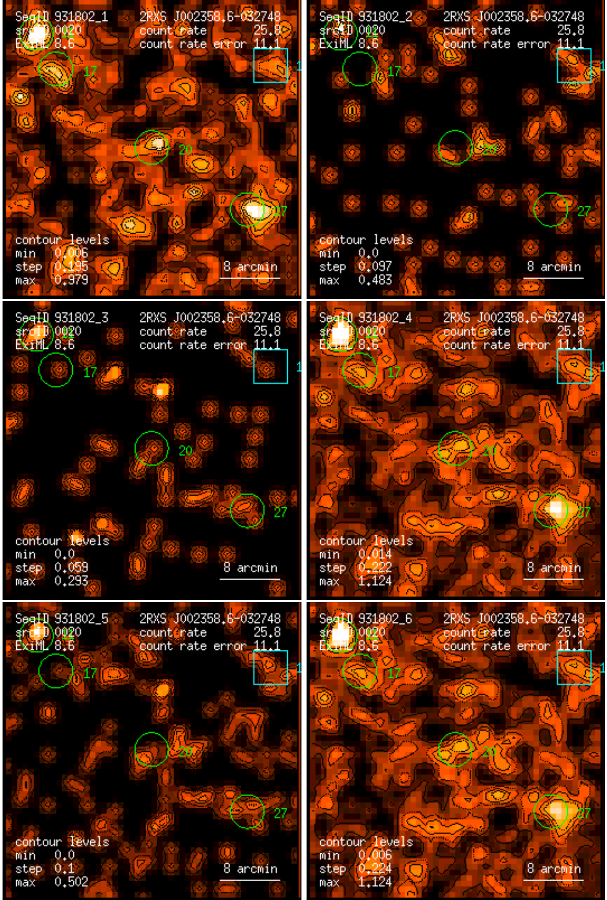
Figure 20: RASS 931802: detection 0020: band rate images, Gaussian filter: (1) PSPC channels 11 – 41, (2) 52 – 90, (3) 91 – 201, (4) 11 – 235, (5) 52 – 201, (6) 11 – 201. Broad band rates in counts/ks. Band rate contour levels in counts/ks/arcmin 2 .
