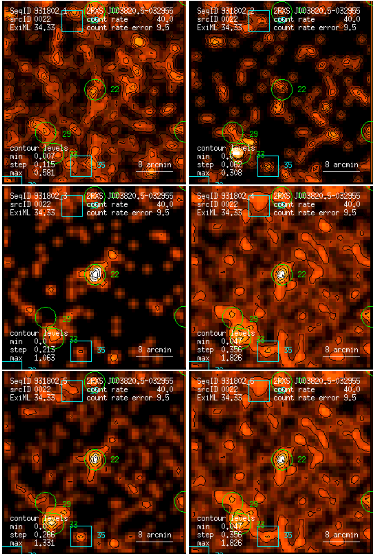
Figure 22: RASS 931802: detection 0022: band rate images, Gaussian filter: (1) PSPC channels 11 – 41, (2) 52 – 90, (3) 91 – 201, (4) 11 – 235, (5) 52 – 201, (6) 11 – 201. Broad band rates in counts/ks. Band rate contour levels in counts/ks/arcmin 2 .
