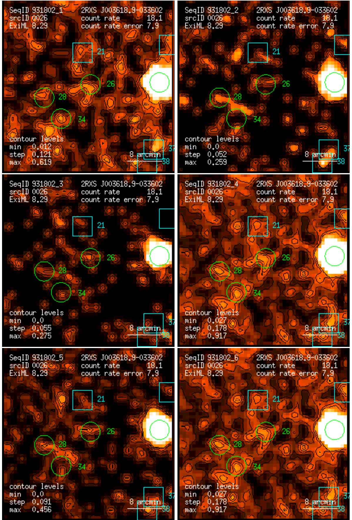
Figure 26: RASS 931802: detection 0026: band rate images, Gaussian filter: (1) PSPC channels 11 – 41, (2) 52 – 90, (3) 91 – 201, (4) 11 – 235, (5) 52 – 201, (6) 11 – 201. Broad band rates in counts/ks. Band rate contour levels in counts/ks/arcmin 2 .
