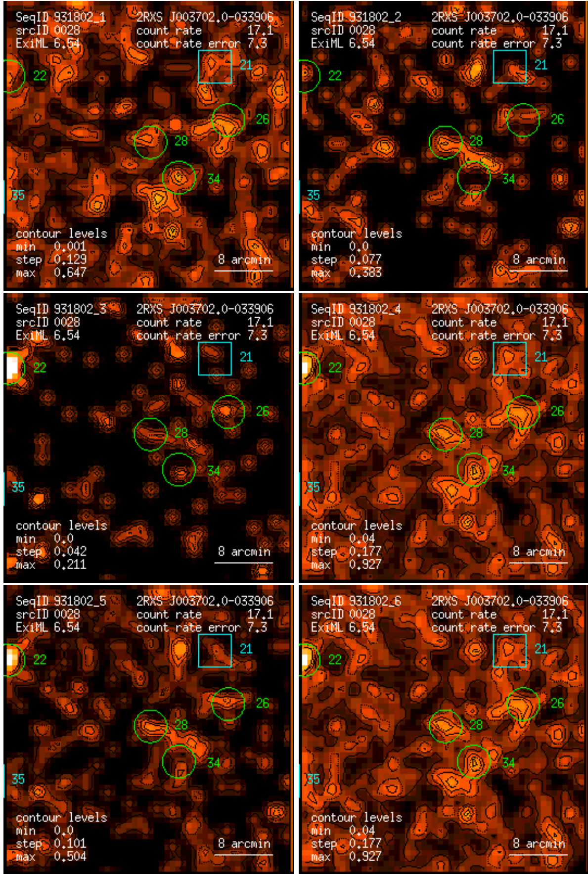
Figure 28: RASS 931802: detection 0028: band rate images, Gaussian filter: (1) PSPC channels 11 – 41, (2) 52 – 90, (3) 91 – 201, (4) 11 – 235, (5) 52 – 201, (6) 11 – 201. Broad band rates in counts/ks. Band rate contour levels in counts/ks/arcmin 2 .
