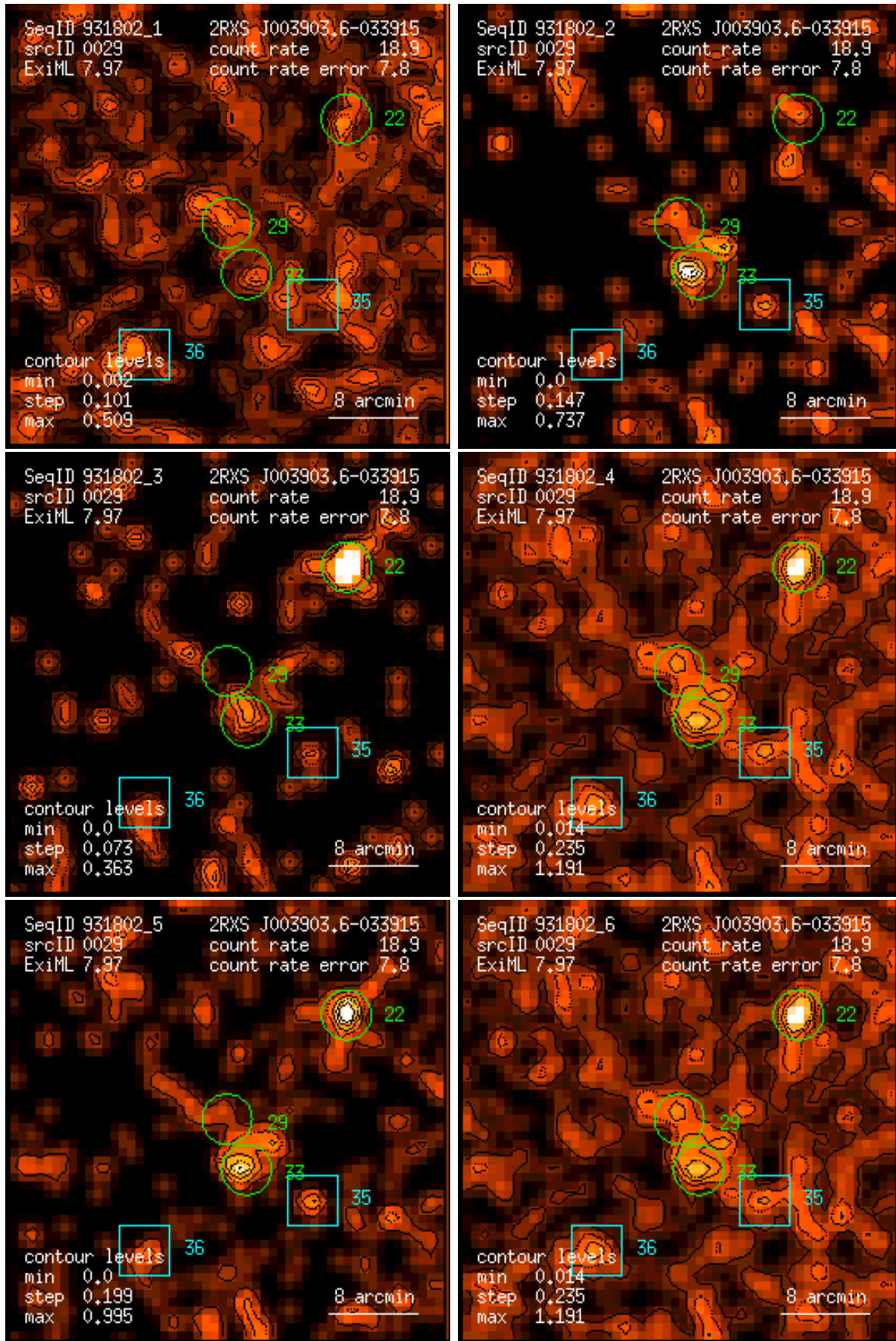
Figure 29: RASS 931802: detection 0029: band rate images, Gaussian filter: (1) PSPC channels 11 – 41, (2) 52 – 90, (3) 91 – 201, (4) 11 – 235, (5) 52 – 201, (6) 11 – 201. Broad band rates in counts/ks. Band rate contour levels in counts/ks/arcmin 2 .
