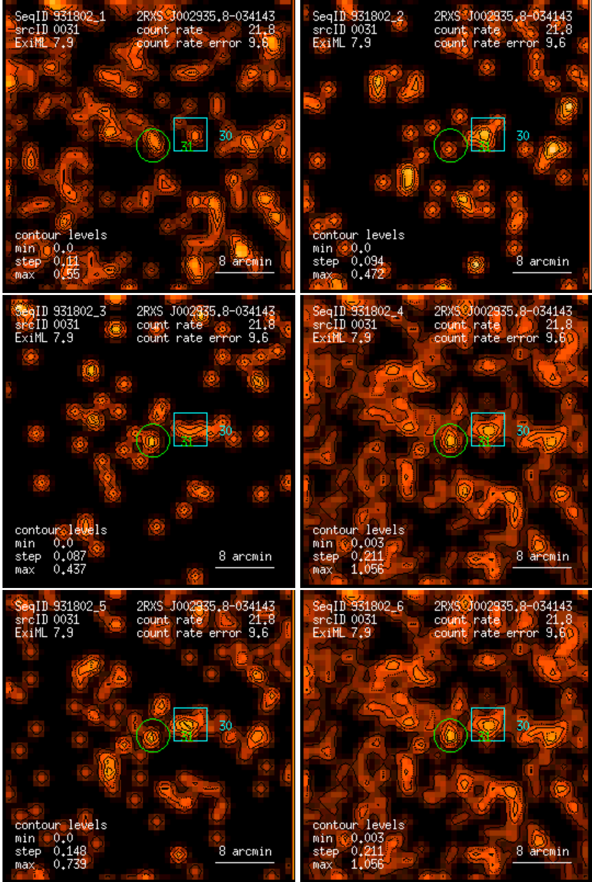
Figure 31: RASS 931802: detection 0031: band rate images, Gaussian filter: (1) PSPC channels 11 – 41, (2) 52 – 90, (3) 91 – 201, (4) 11 – 235, (5) 52 – 201, (6) 11 – 201. Broad band rates in counts/ks. Band rate contour levels in counts/ks/arcmin 2 .
