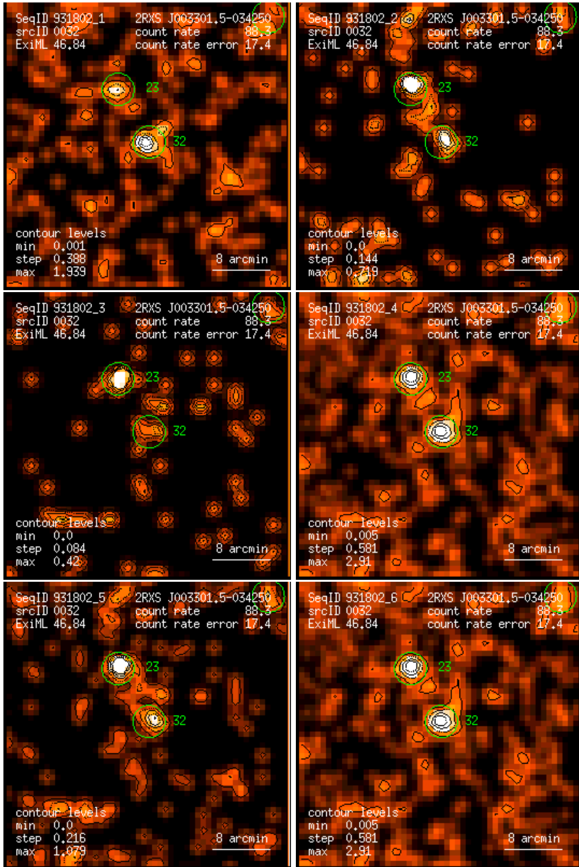
Figure 32: RASS 931802: detection 0032: band rate images, Gaussian filter: (1) PSPC channels 11 – 41, (2) 52 – 90, (3) 91 – 201, (4) 11 – 235, (5) 52 – 201, (6) 11 – 201. Broad band rates in counts/ks. Band rate contour levels in counts/ks/arcmin 2 .
