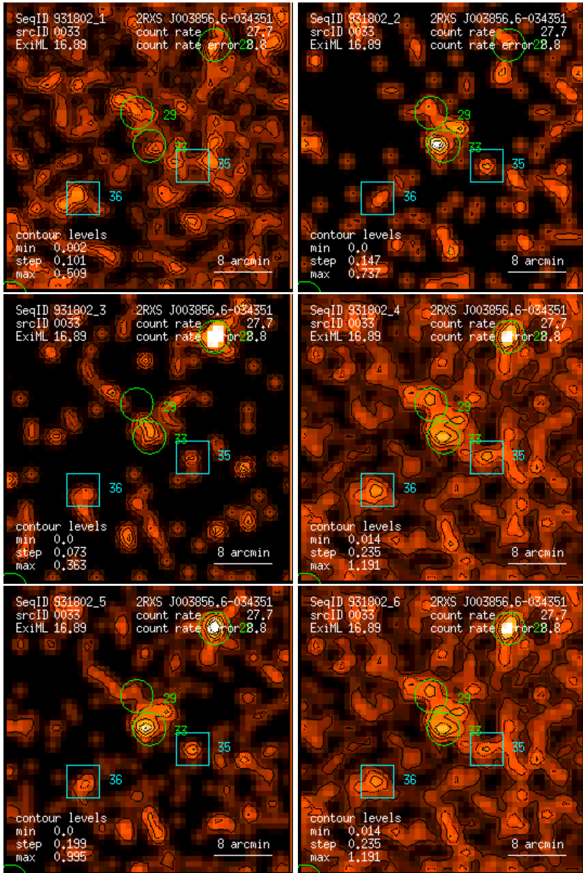
Figure 33: RASS 931802: detection 0033: band rate images, Gaussian filter: (1) PSPC channels 11 – 41, (2) 52 – 90, (3) 91 – 201, (4) 11 – 235, (5) 52 – 201, (6) 11 – 201. Broad band rates in counts/ks. Band rate contour levels in counts/ks/arcmin 2 .
