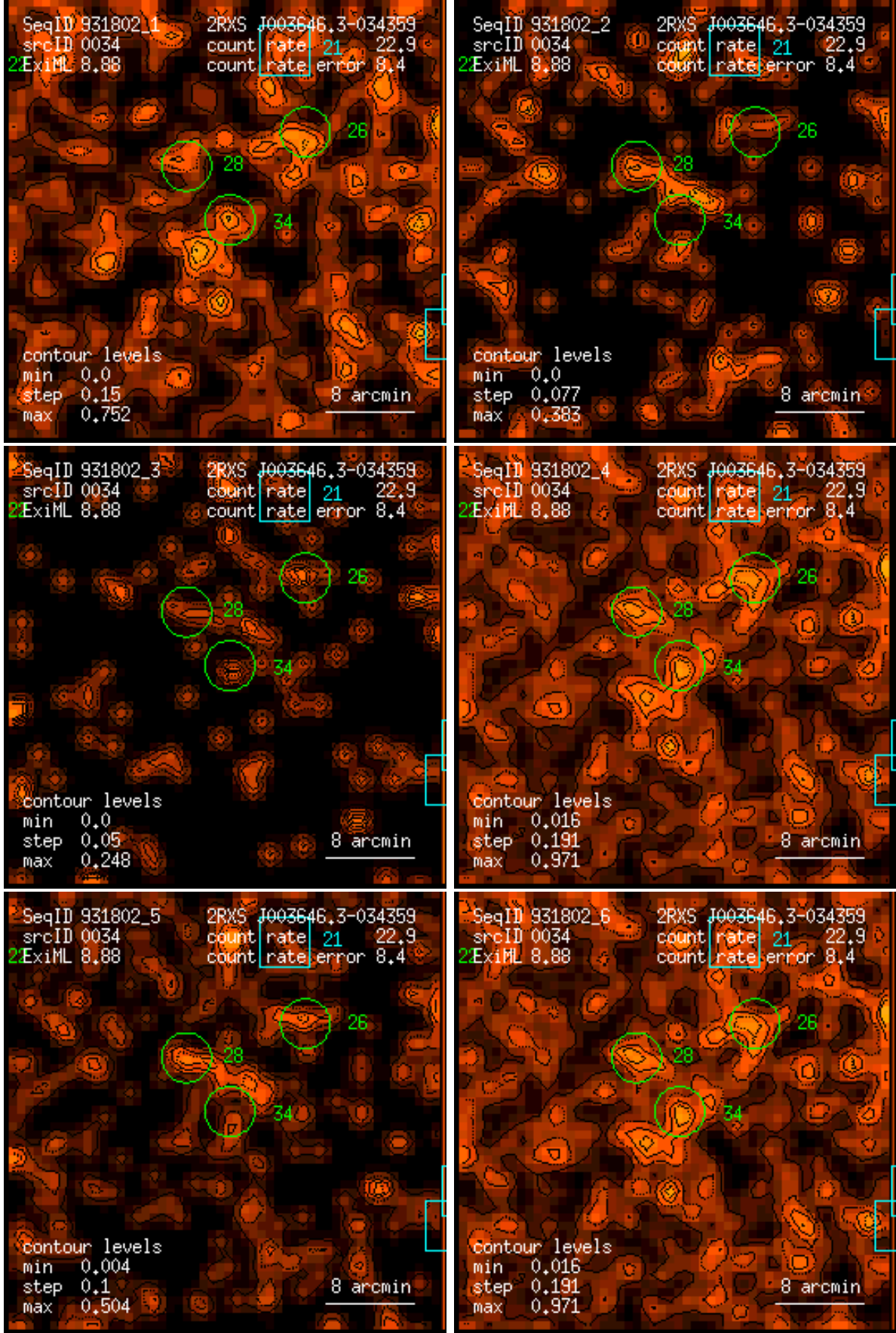
Figure 34: RASS 931802: detection 0034: band rate images, Gaussian filter: (1) PSPC channels 11 – 41, (2) 52 – 90, (3) 91 – 201, (4) 11 – 235, (5) 52 – 201, (6) 11 – 201. Broad band rates in counts/ks. Band rate contour levels in counts/ks/arcmin 2 .
