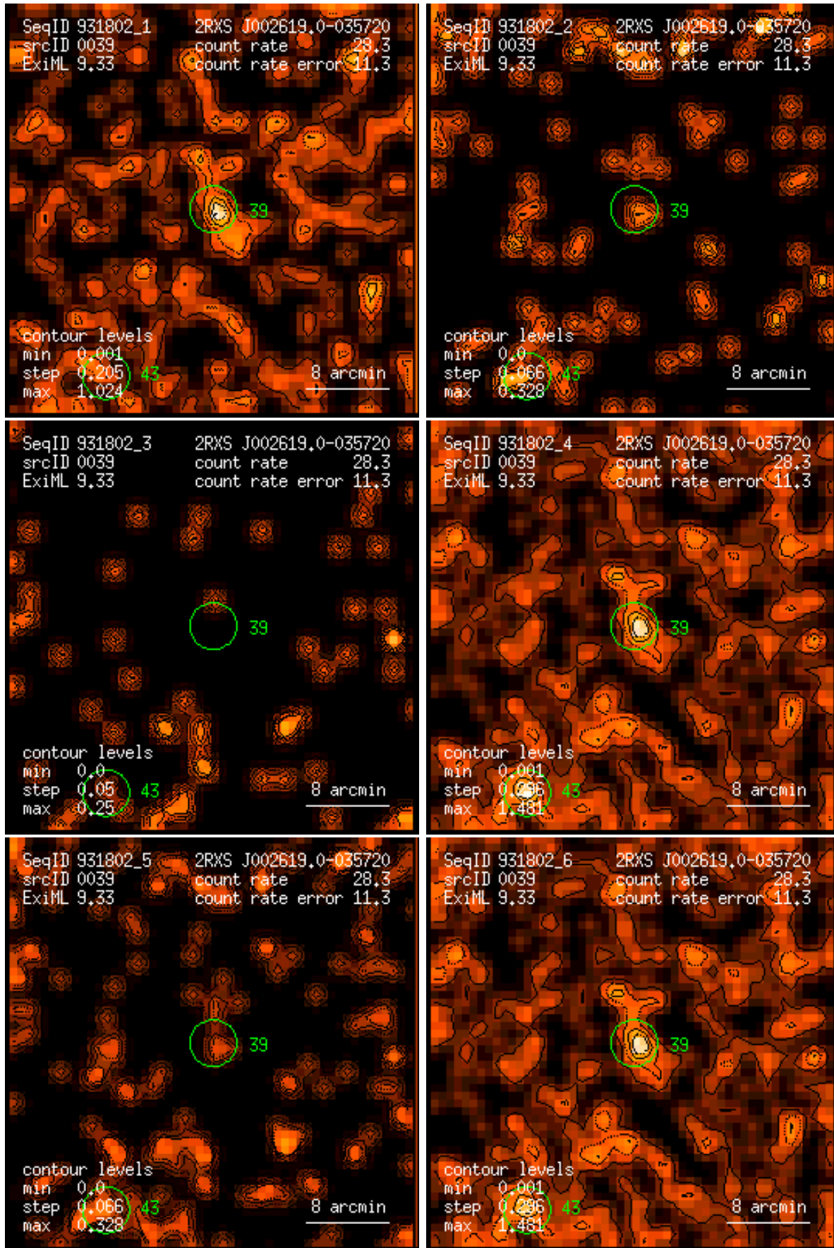
Figure 39: RASS 931802: detection 0039: band rate images, Gaussian filter: (1) PSPC channels 11 – 41, (2) 52 – 90, (3) 91 – 201, (4) 11 – 235, (5) 52 – 201, (6) 11 – 201. Broad band rates in counts/ks. Band rate contour levels in counts/ks/arcmin 2 .
