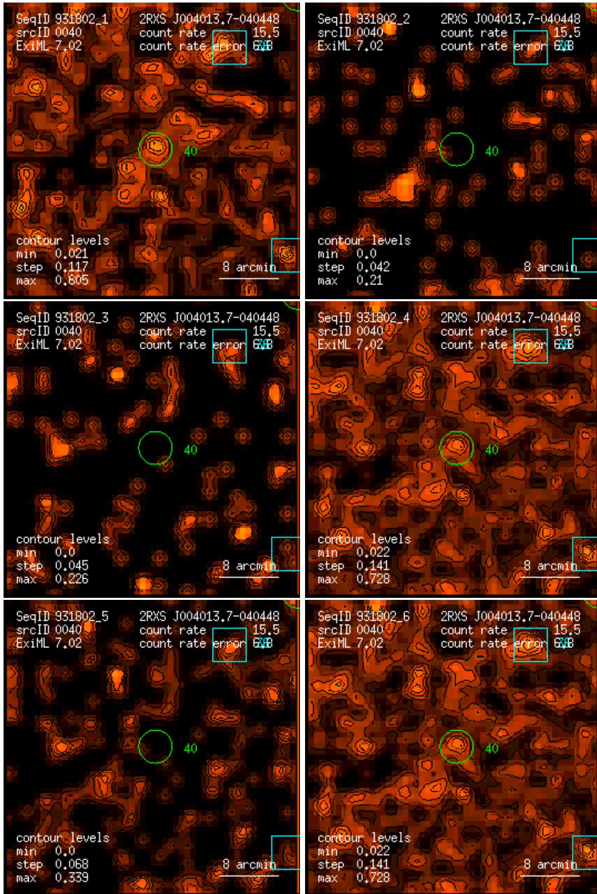
Figure 40: RASS 931802: detection 0040: band rate images, Gaussian filter: (1) PSPC channels 11 – 41, (2) 52 – 90, (3) 91 – 201, (4) 11 – 235, (5) 52 – 201, (6) 11 – 201. Broad band rates in counts/ks. Band rate contour levels in counts/ks/arcmin 2 .
