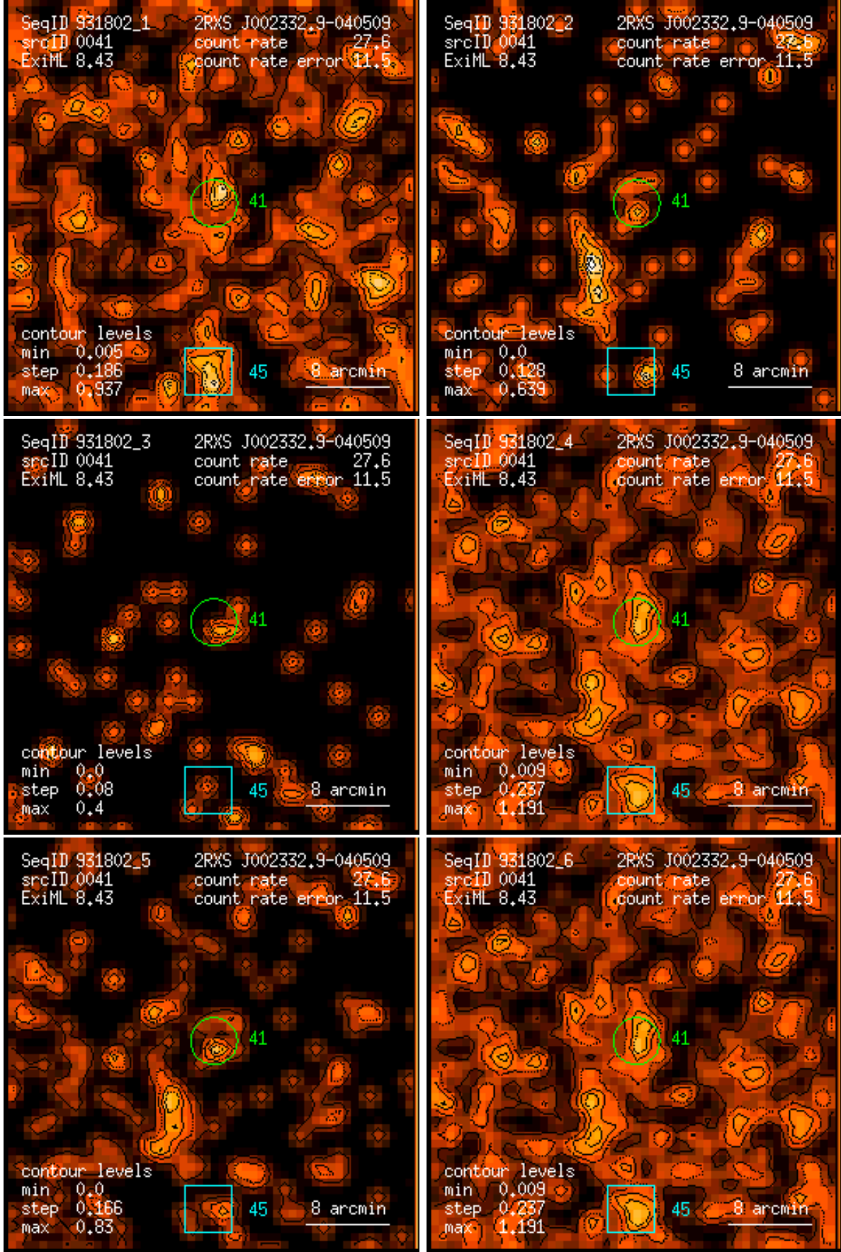
Figure 41: RASS 931802: detection 0041: band rate images, Gaussian filter: (1) PSPC channels 11 – 41, (2) 52 – 90, (3) 91 – 201, (4) 11 – 235, (5) 52 – 201, (6) 11 – 201. Broad band rates in counts/ks. Band rate contour levels in counts/ks/arcmin 2 .
