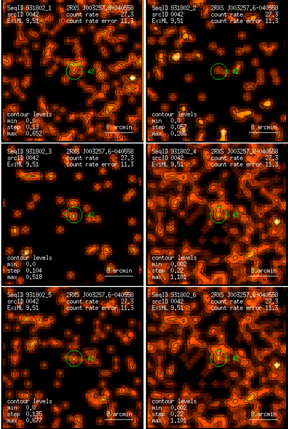
Figure 42: RASS 931802: detection 0042: band rate images, Gaussian filter: (1) PSPC channels 11 – 41, (2) 52 – 90, (3) 91 – 201, (4) 11 – 235, (5) 52 – 201, (6) 11 – 201. Broad band rates in counts/ks. Band rate contour levels in counts/ks/arcmin 2 .
