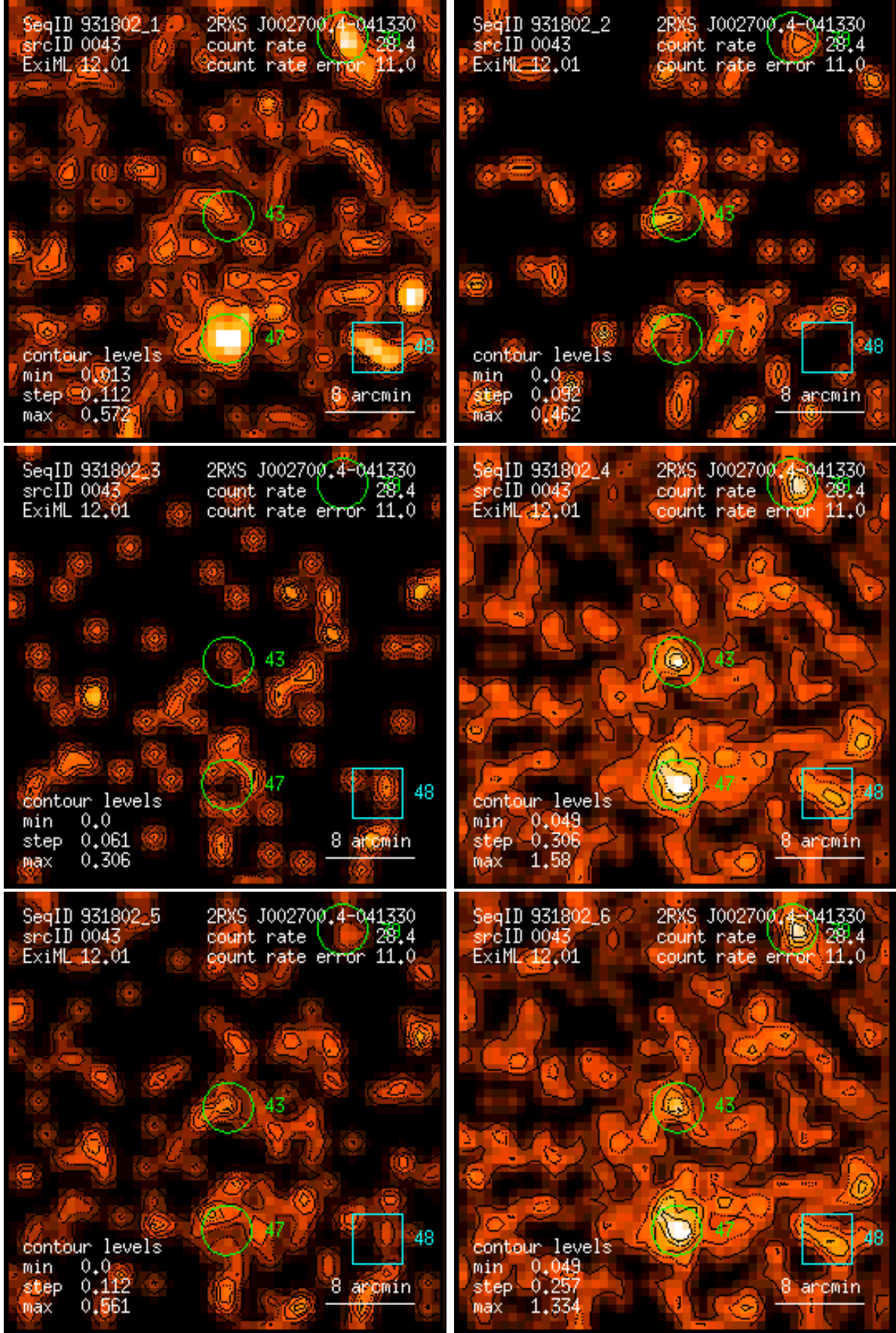
Figure 43: RASS 931802: detection 0043: band rate images, Gaussian filter: (1) PSPC channels 11 – 41, (2) 52 – 90, (3) 91 – 201, (4) 11 – 235, (5) 52 – 201, (6) 11 – 201. Broad band rates in counts/ks. Band rate contour levels in counts/ks/arcmin 2 .
