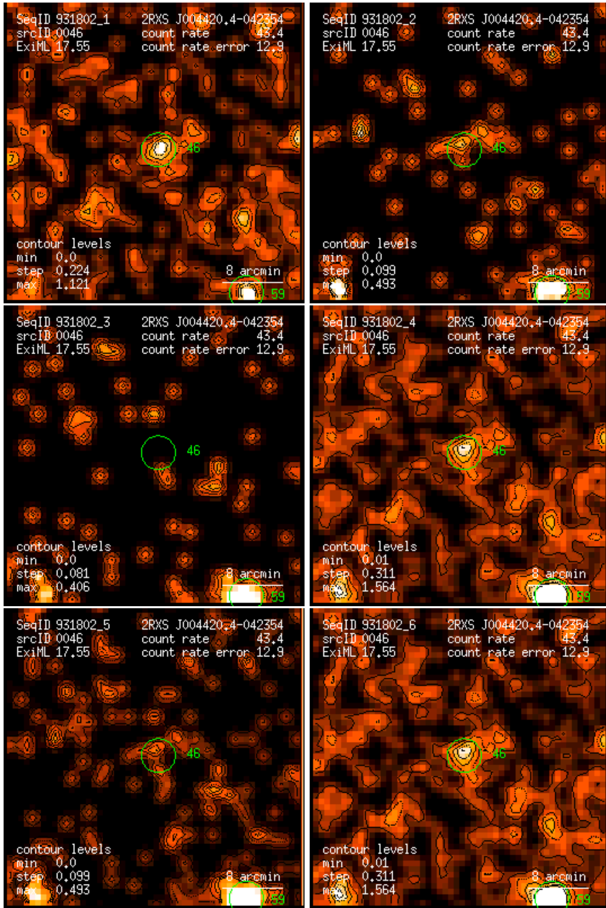
Figure 46: RASS 931802: detection 0046: band rate images, Gaussian filter: (1) PSPC channels 11 – 41, (2) 52 – 90, (3) 91 – 201, (4) 11 – 235, (5) 52 – 201, (6) 11 – 201. Broad band rates in counts/ks. Band rate contour levels in counts/ks/arcmin 2 .
