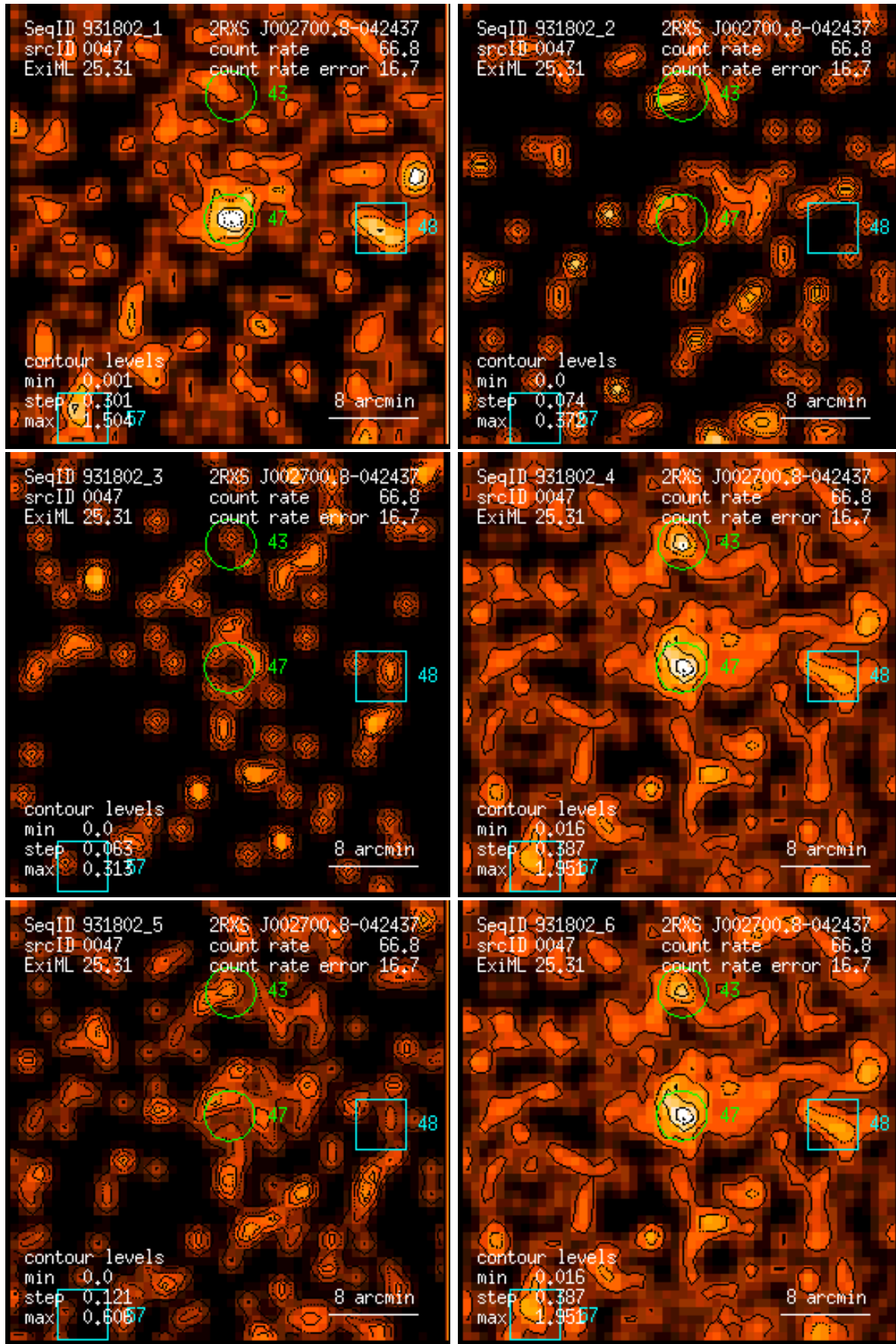
Figure 47: RASS 931802: detection 0047: band rate images, Gaussian filter: (1) PSPC channels 11 – 41, (2) 52 – 90, (3) 91 – 201, (4) 11 – 235, (5) 52 – 201, (6) 11 – 201. Broad band rates in counts/ks. Band rate contour levels in counts/ks/arcmin 2 .
