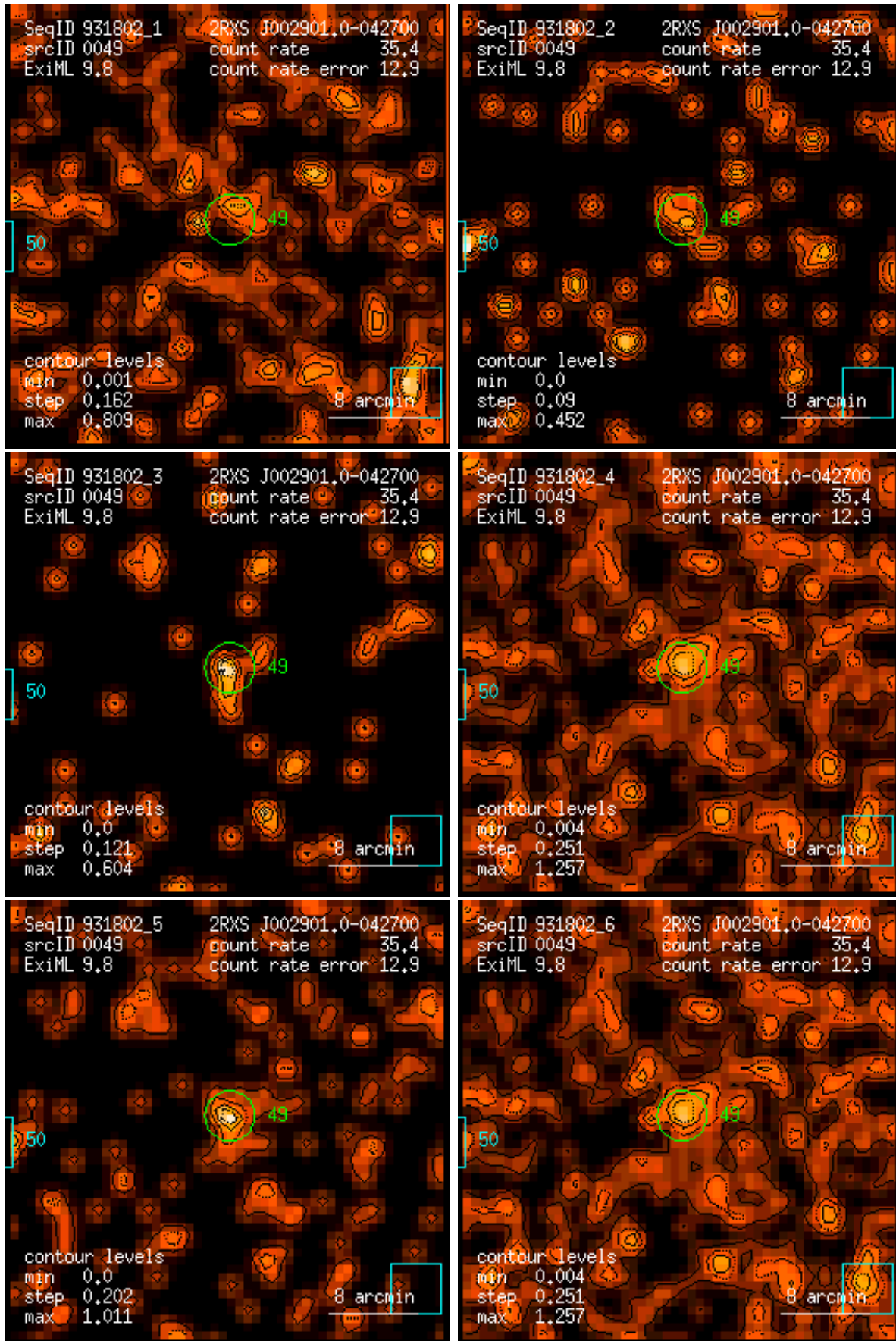
Figure 49: RASS 931802: detection 0049: band rate images, Gaussian filter: (1) PSPC channels 11 – 41, (2) 52 – 90, (3) 91 – 201, (4) 11 – 235, (5) 52 – 201, (6) 11 – 201. Broad band rates in counts/ks. Band rate contour levels in counts/ks/arcmin 2 .
