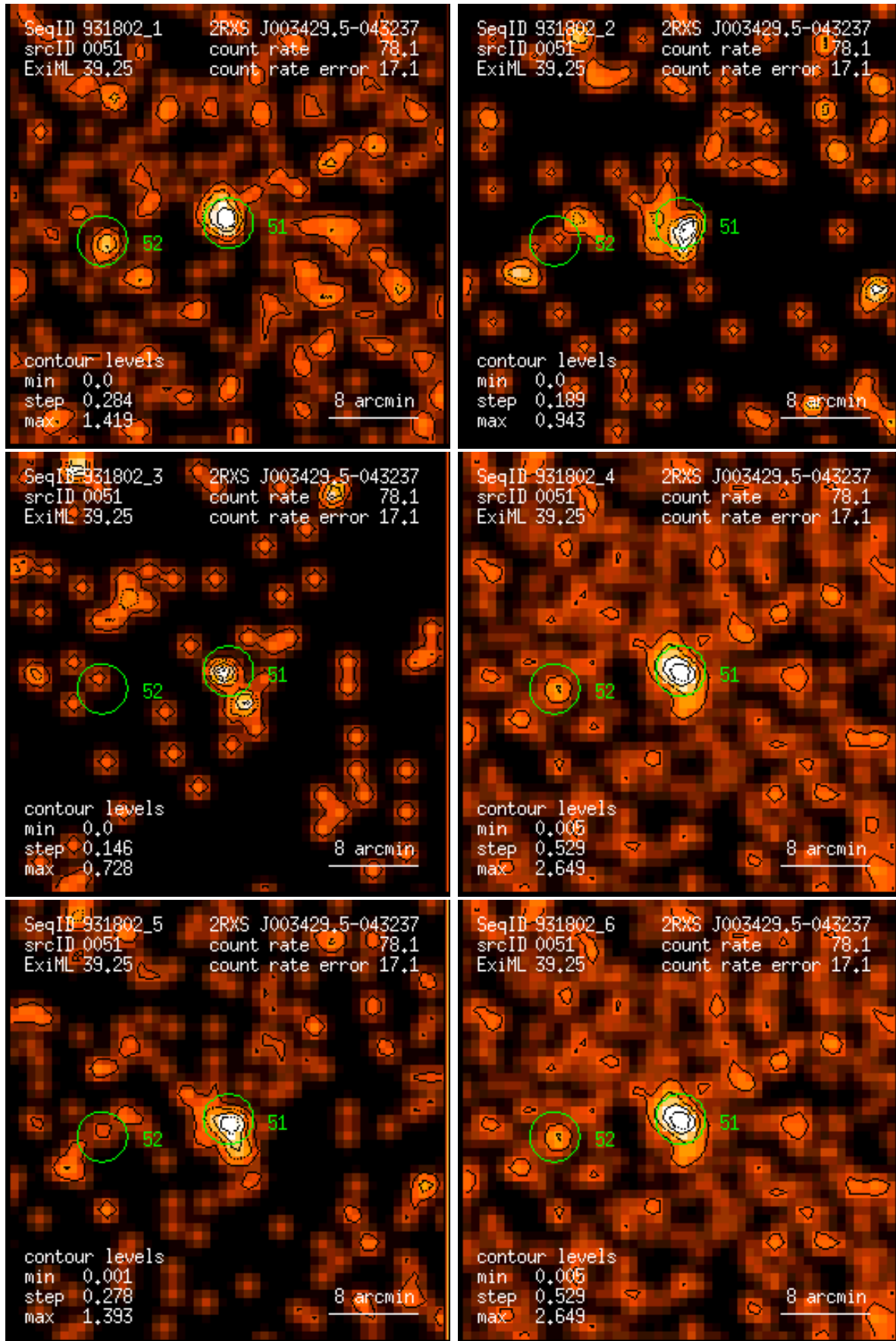
Figure 51: RASS 931802: detection 0051: band rate images, Gaussian filter: (1) PSPC channels 11 – 41, (2) 52 – 90, (3) 91 – 201, (4) 11 – 235, (5) 52 – 201, (6) 11 – 201. Broad band rates in counts/ks. Band rate contour levels in counts/ks/arcmin 2 .
