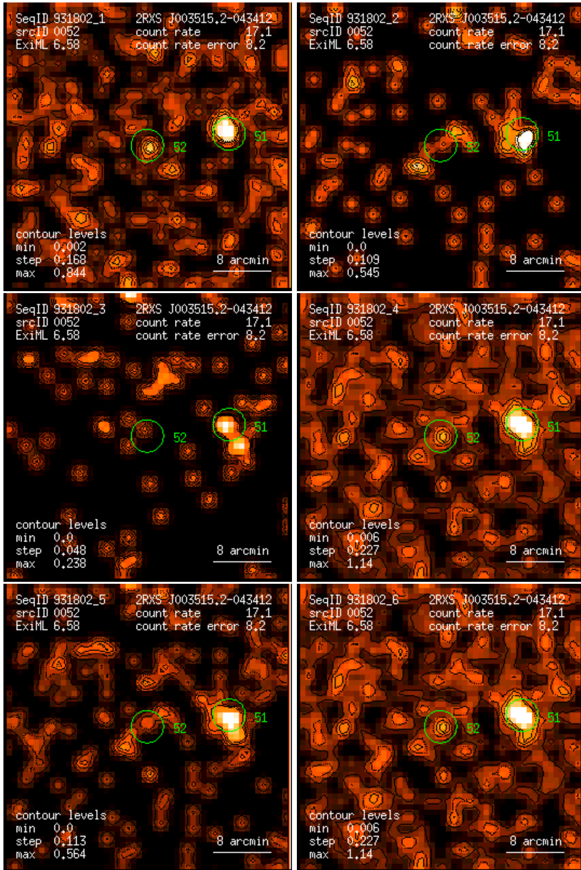
Figure 52: RASS 931802: detection 0052: band rate images, Gaussian filter: (1) PSPC channels 11 – 41, (2) 52 – 90, (3) 91 – 201, (4) 11 – 235, (5) 52 – 201, (6) 11 – 201. Broad band rates in counts/ks. Band rate contour levels in counts/ks/arcmin 2 .
