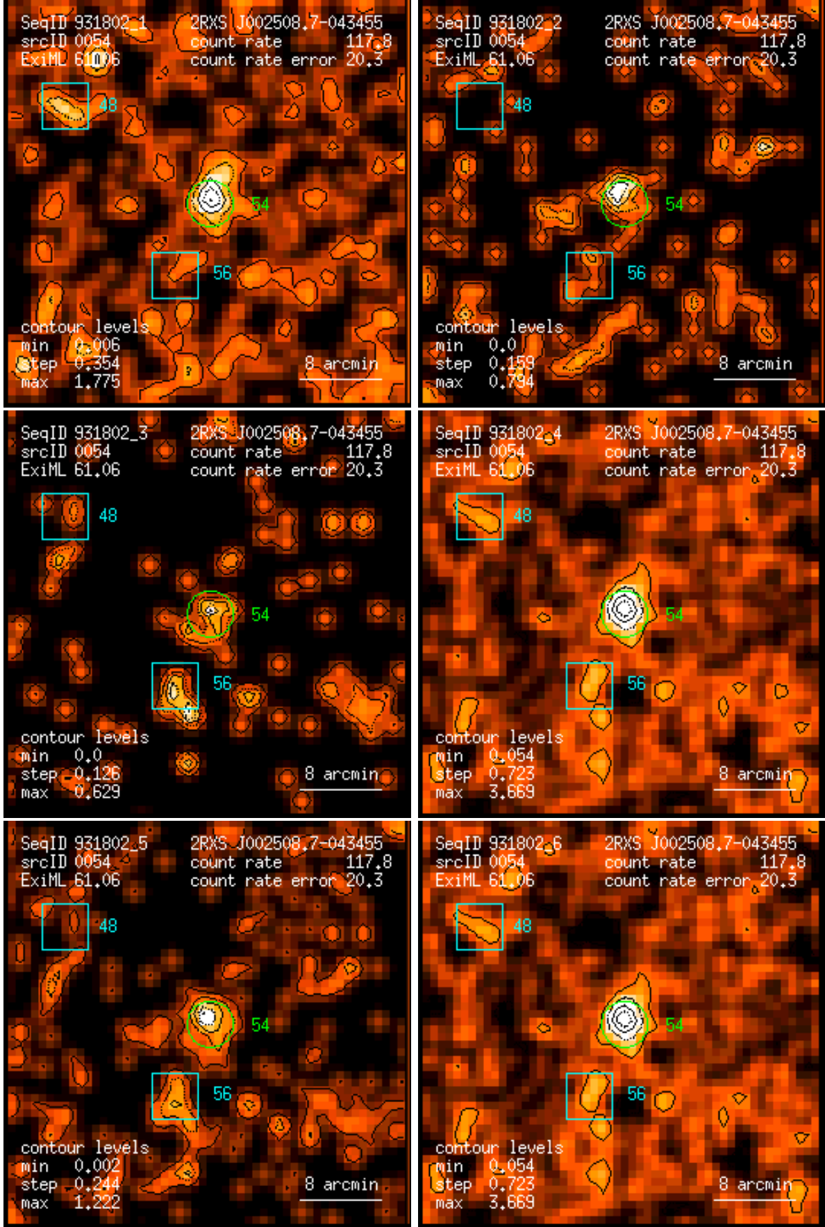
Figure 54: RASS 931802: detection 0054: band rate images, Gaussian filter: (1) PSPC channels 11 – 41, (2) 52 – 90, (3) 91 – 201, (4) 11 – 235, (5) 52 – 201, (6) 11 – 201. Broad band rates in counts/ks. Band rate contour levels in counts/ks/arcmin 2 .
