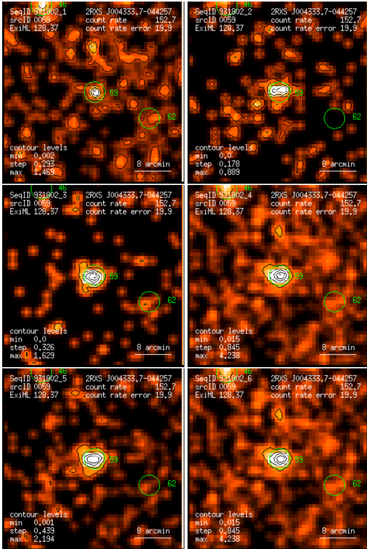
Figure 59: RASS 931802: detection 0059: band rate images, Gaussian filter: (1) PSPC channels 11 – 41, (2) 52 – 90, (3) 91 – 201, (4) 11 – 235, (5) 52 – 201, (6) 11 – 201. Broad band rates in counts/ks. Band rate contour levels in counts/ks/arcmin 2 .
