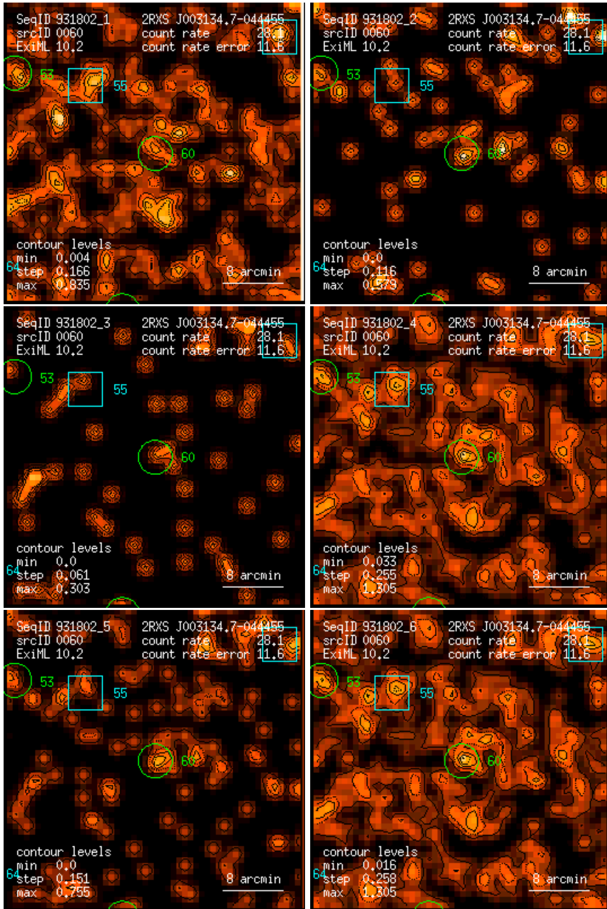
Figure 60: RASS 931802: detection 0060: band rate images, Gaussian filter: (1) PSPC channels 11 – 41, (2) 52 – 90, (3) 91 – 201, (4) 11 – 235, (5) 52 – 201, (6) 11 – 201. Broad band rates in counts/ks. Band rate contour levels in counts/ks/arcmin 2 .
