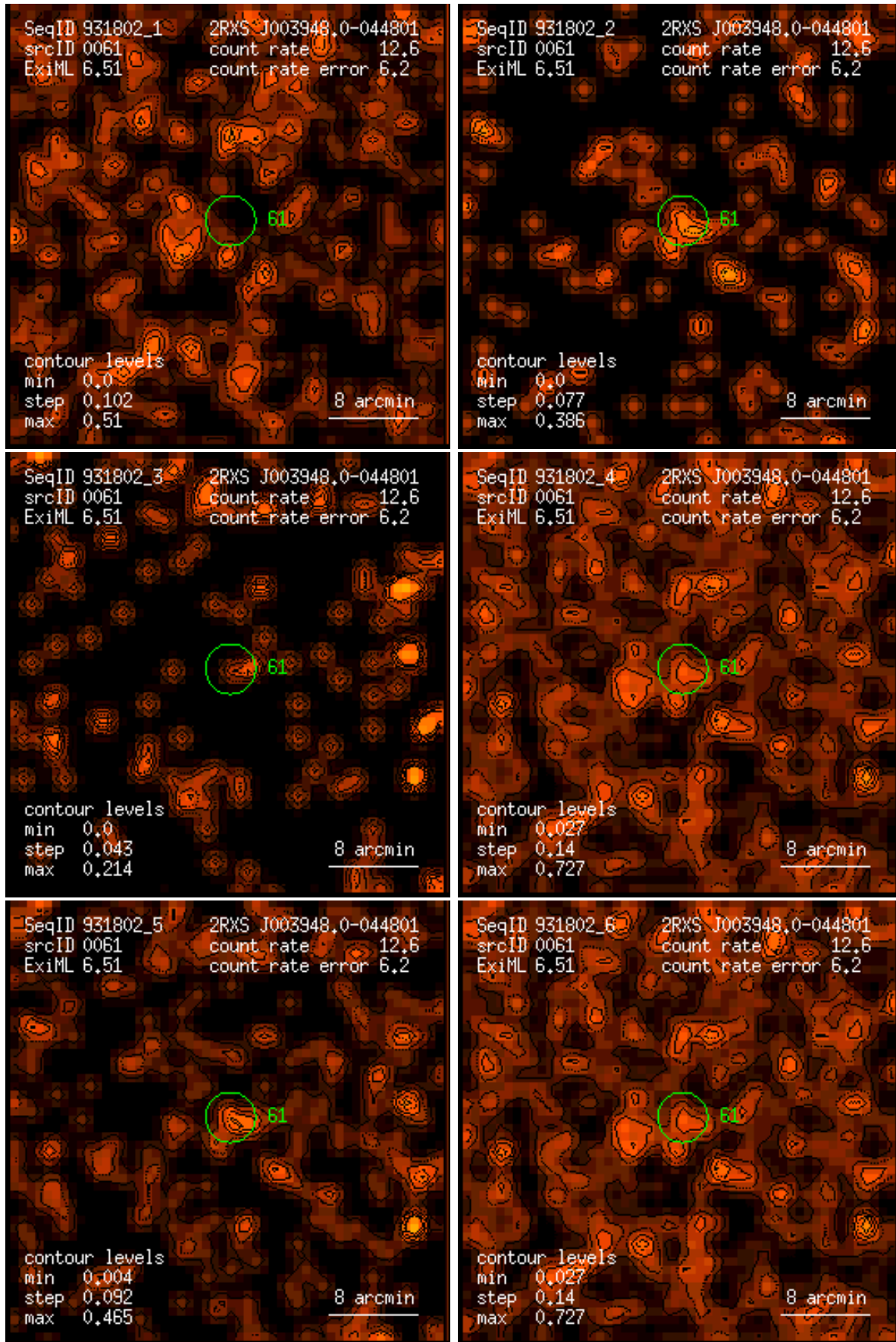
Figure 61: RASS 931802: detection 0061: band rate images, Gaussian filter: (1) PSPC channels 11 – 41, (2) 52 – 90, (3) 91 – 201, (4) 11 – 235, (5) 52 – 201, (6) 11 – 201. Broad band rates in counts/ks. Band rate contour levels in counts/ks/arcmin 2 .
