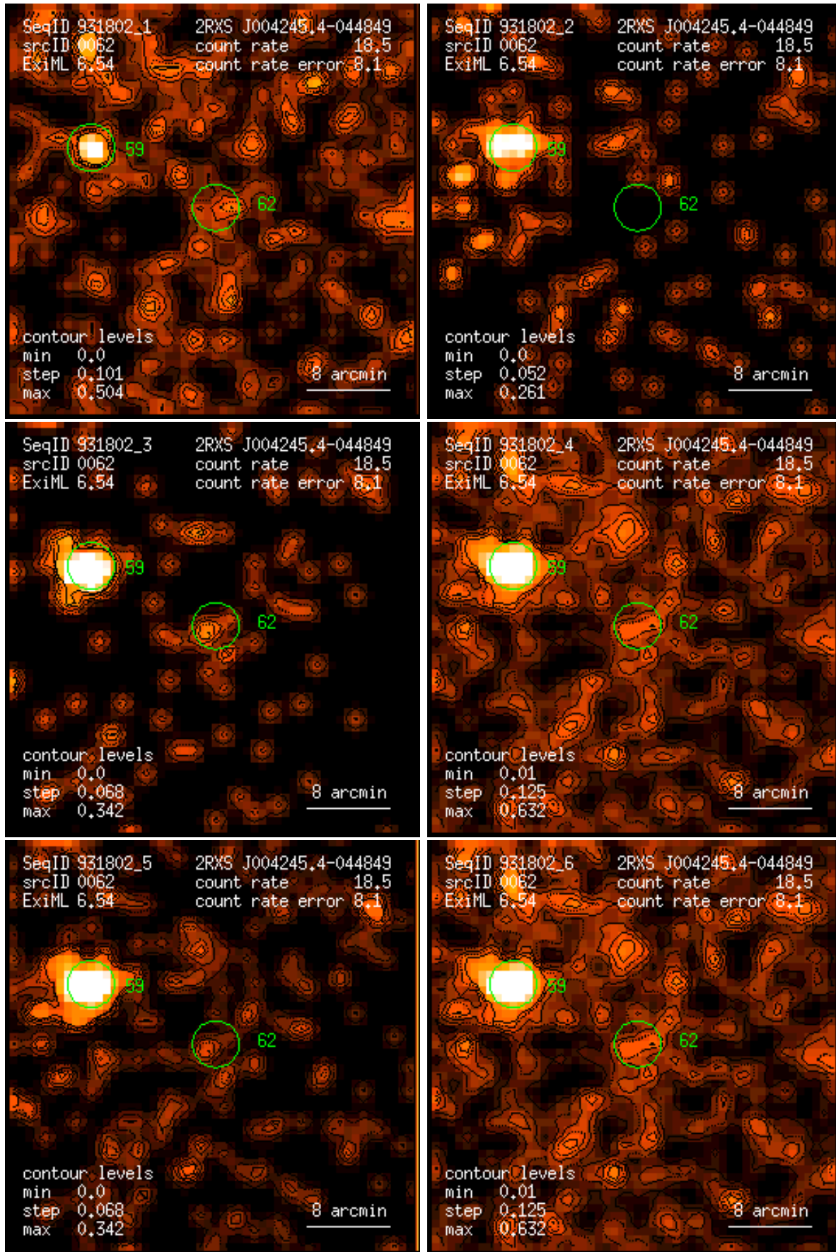
Figure 62: RASS 931802: detection 0062: band rate images, Gaussian filter: (1) PSPC channels 11 – 41, (2) 52 – 90, (3) 91 – 201, (4) 11 – 235, (5) 52 – 201, (6) 11 – 201. Broad band rates in counts/ks. Band rate contour levels in counts/ks/arcmin 2 .
