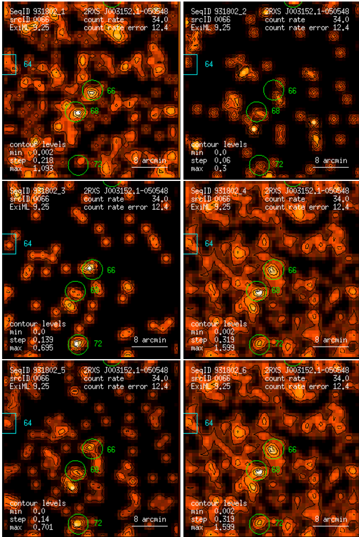
Figure 66: RASS 931802: detection 0066: band rate images, Gaussian filter: (1) PSPC channels 11 – 41, (2) 52 – 90, (3) 91 – 201, (4) 11 – 235, (5) 52 – 201, (6) 11 – 201. Broad band rates in counts/ks. Band rate contour levels in counts/ks/arcmin 2 .
