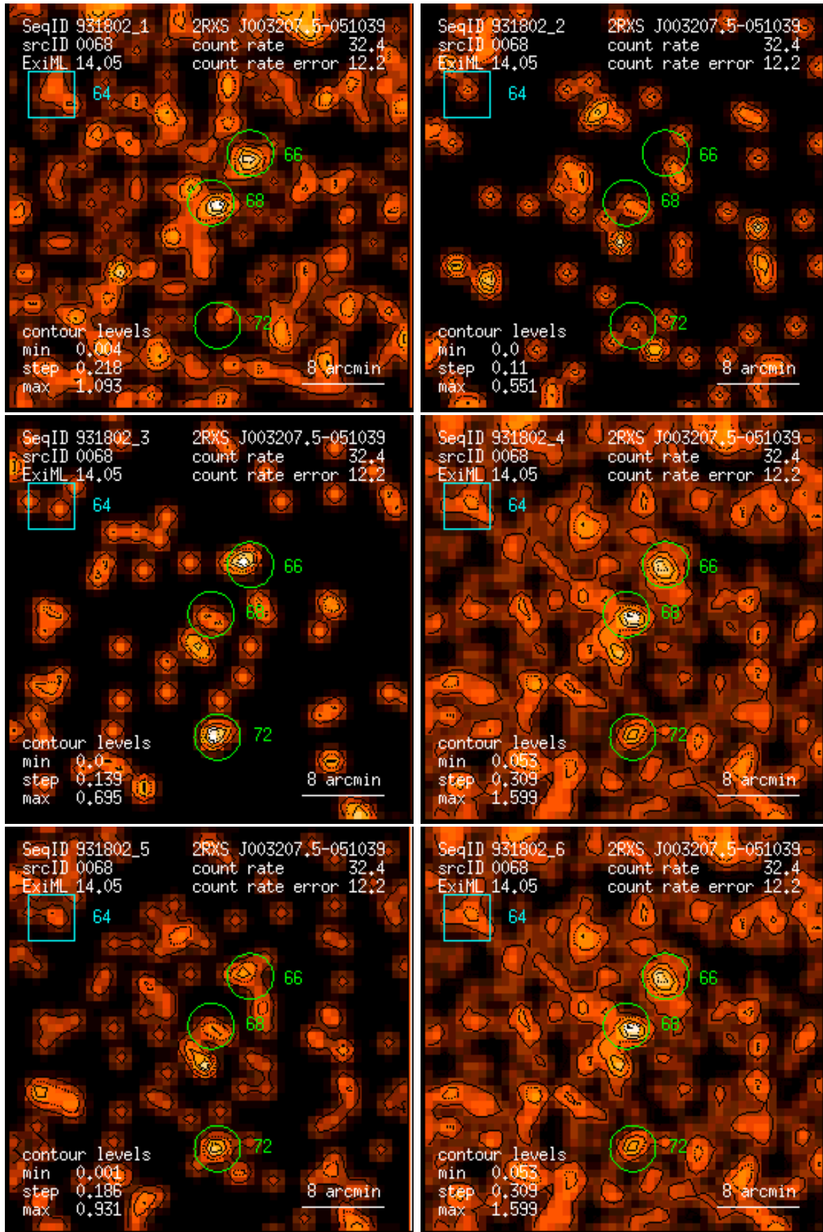
Figure 68: RASS 931802: detection 0068: band rate images, Gaussian filter: (1) PSPC channels 11 – 41, (2) 52 – 90, (3) 91 – 201, (4) 11 – 235, (5) 52 – 201, (6) 11 – 201. Broad band rates in counts/ks. Band rate contour levels in counts/ks/arcmin 2 .
