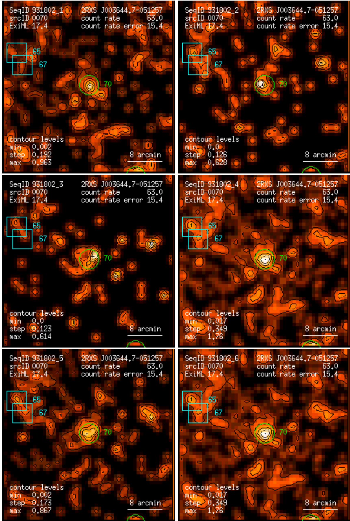
Figure 70: RASS 931802: detection 0070: band rate images, Gaussian filter: (1) PSPC channels 11 – 41, (2) 52 – 90, (3) 91 – 201, (4) 11 – 235, (5) 52 – 201, (6) 11 – 201. Broad band rates in counts/ks. Band rate contour levels in counts/ks/arcmin 2 .
