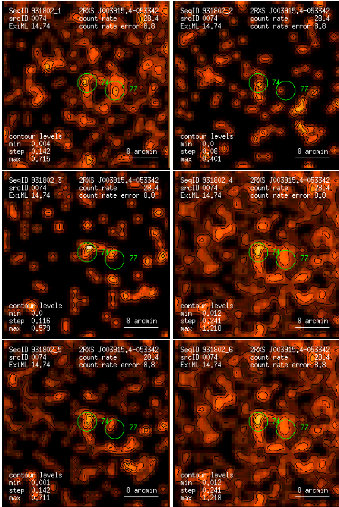
Figure 74: RASS 931802: detection 0074: band rate images, Gaussian filter: (1) PSPC channels 11 – 41, (2) 52 – 90, (3) 91 – 201, (4) 11 – 235, (5) 52 – 201, (6) 11 – 201. Broad band rates in counts/ks. Band rate contour levels in counts/ks/arcmin 2 .
