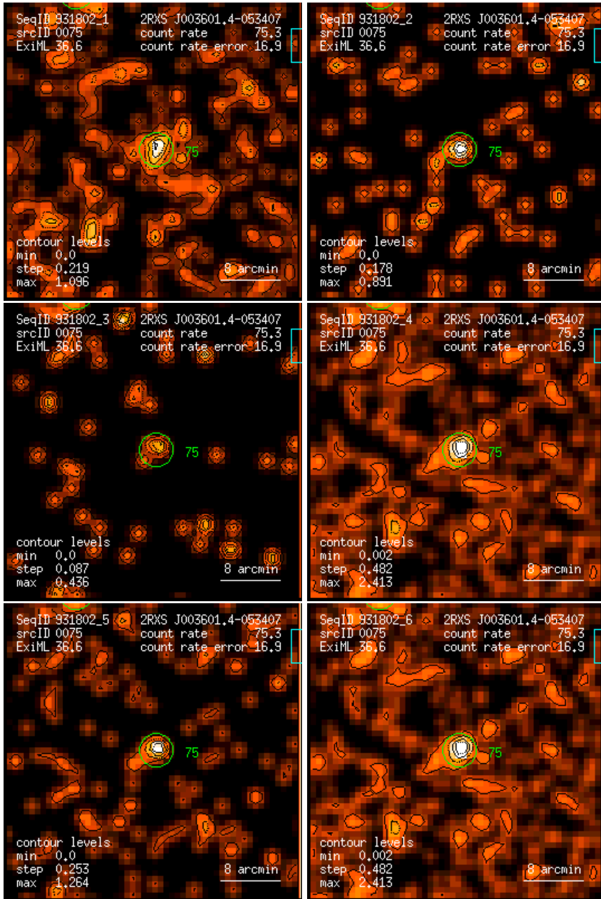
Figure 75: RASS 931802: detection 0075: band rate images, Gaussian filter: (1) PSPC channels 11 – 41, (2) 52 – 90, (3) 91 – 201, (4) 11 – 235, (5) 52 – 201, (6) 11 – 201. Broad band rates in counts/ks. Band rate contour levels in counts/ks/arcmin 2 .
