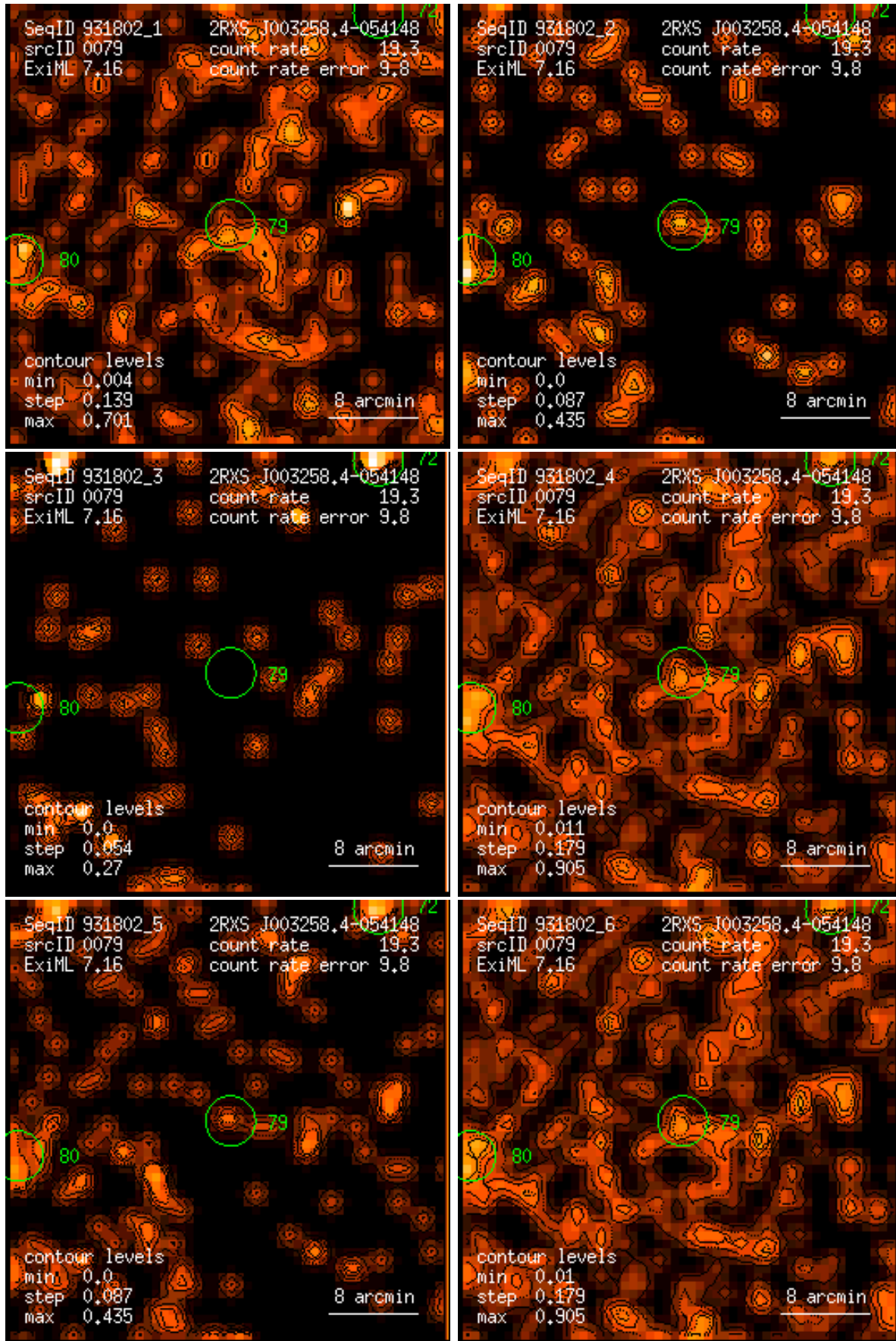
Figure 79: RASS 931802: detection 0079: band rate images, Gaussian filter: (1) PSPC channels 11 – 41, (2) 52 – 90, (3) 91 – 201, (4) 11 – 235, (5) 52 – 201, (6) 11 – 201. Broad band rates in counts/ks. Band rate contour levels in counts/ks/arcmin 2 .
