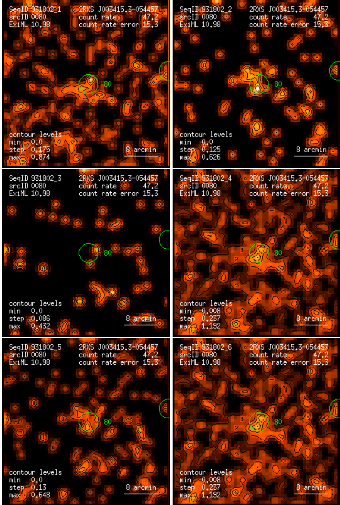
Figure 80: RASS 931802: detection 0080: band rate images, Gaussian filter: (1) PSPC channels 11 – 41, (2) 52 – 90, (3) 91 – 201, (4) 11 – 235, (5) 52 – 201, (6) 11 – 201. Broad band rates in counts/ks. Band rate contour levels in counts/ks/arcmin 2 .
