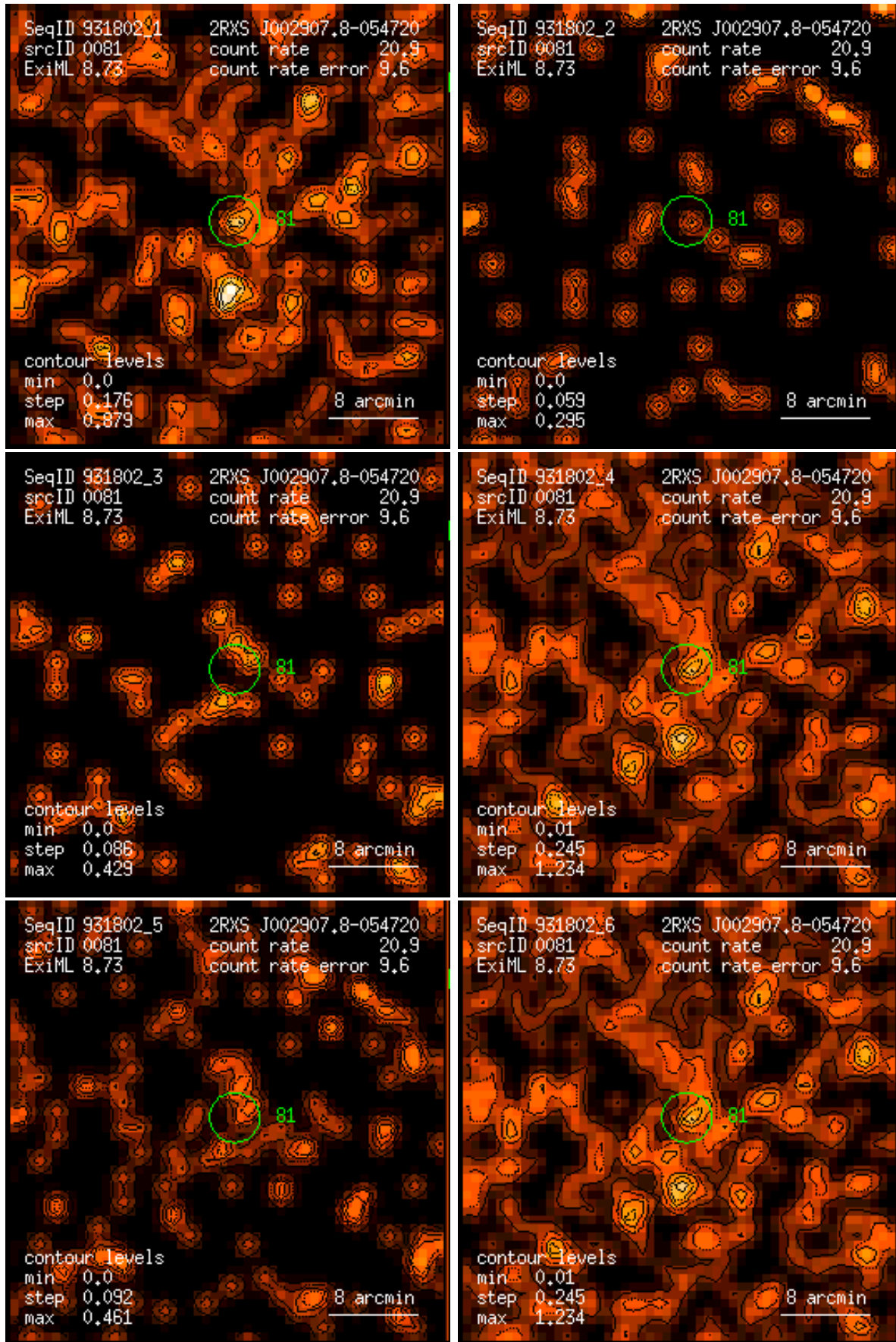
Figure 81: RASS 931802: detection 0081: band rate images, Gaussian filter: (1) PSPC channels 11 – 41, (2) 52 – 90, (3) 91 – 201, (4) 11 – 235, (5) 52 – 201, (6) 11 – 201. Broad band rates in counts/ks. Band rate contour levels in counts/ks/arcmin 2 .
