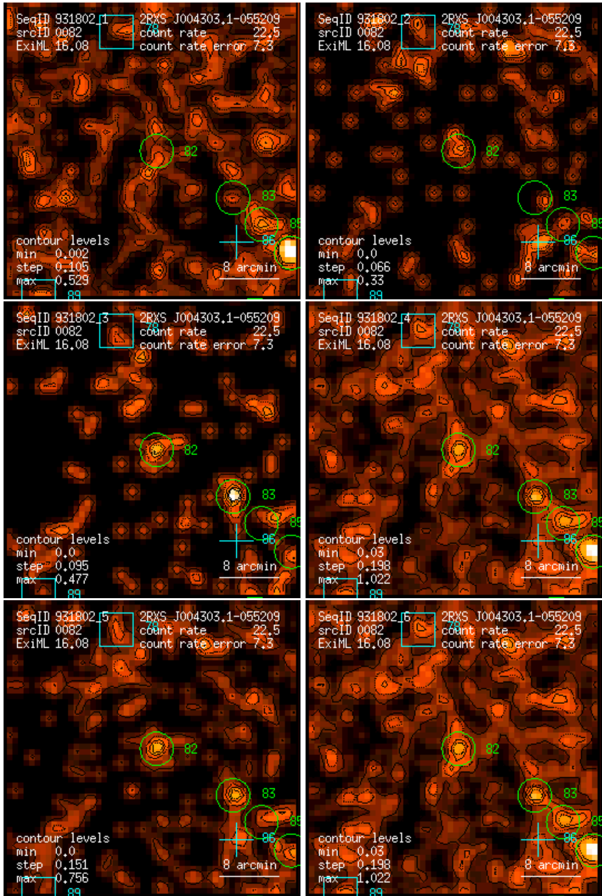
Figure 82: RASS 931802: detection 0082: band rate images, Gaussian filter: (1) PSPC channels 11 – 41, (2) 52 – 90, (3) 91 – 201, (4) 11 – 235, (5) 52 – 201, (6) 11 – 201. Broad band rates in counts/ks. Band rate contour levels in counts/ks/arcmin 2 .
