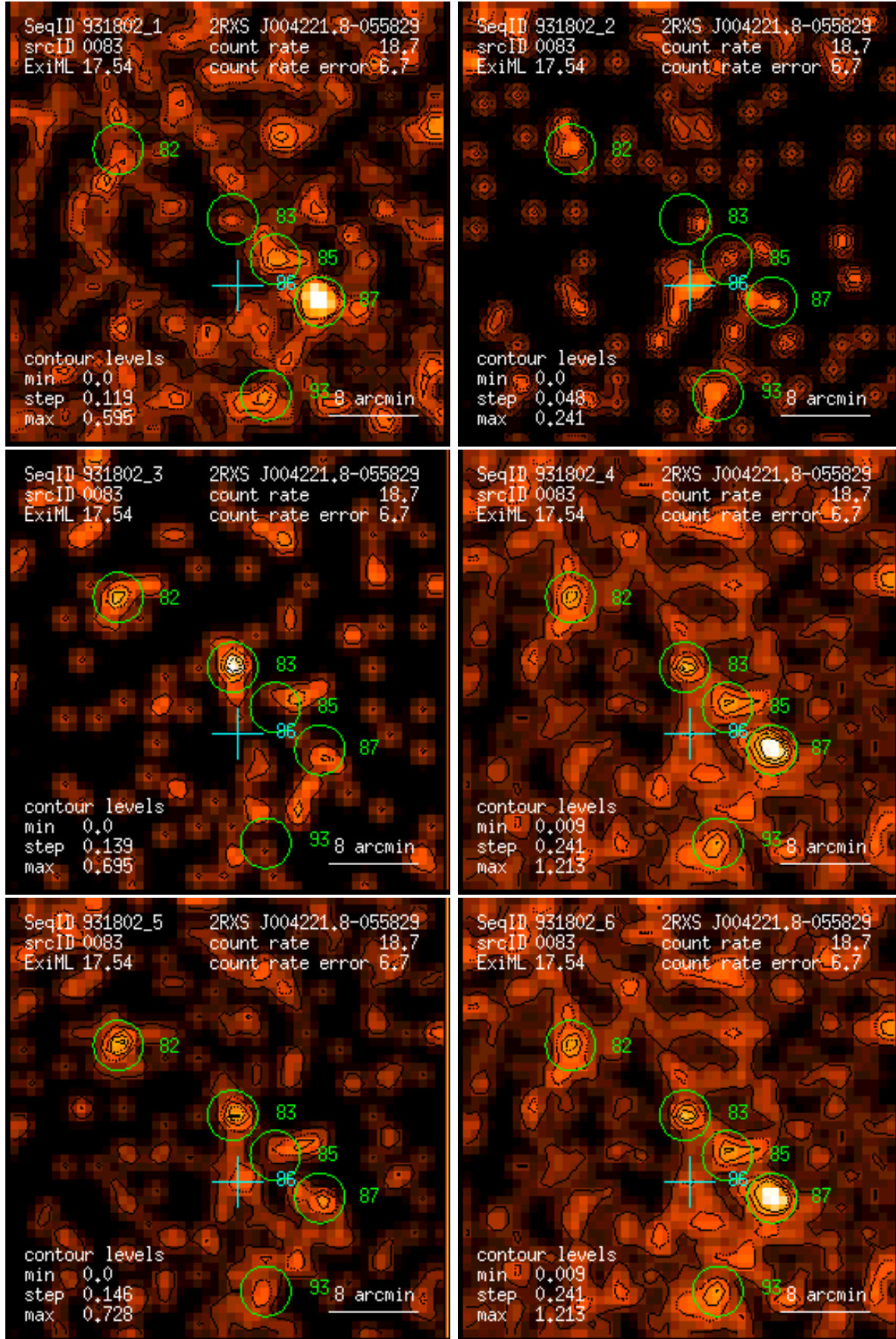
Figure 83: RASS 931802: detection 0083: band rate images, Gaussian filter: (1) PSPC channels 11 – 41, (2) 52 – 90, (3) 91 – 201, (4) 11 – 235, (5) 52 – 201, (6) 11 – 201. Broad band rates in counts/ks. Band rate contour levels in counts/ks/arcmin 2 .
