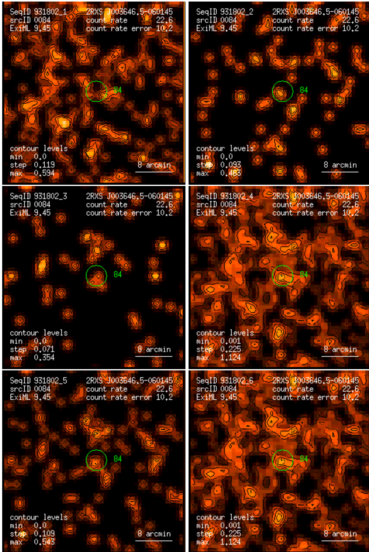
Figure 84: RASS 931802: detection 0084: band rate images, Gaussian filter: (1) PSPC channels 11 – 41, (2) 52 – 90, (3) 91 – 201, (4) 11 – 235, (5) 52 – 201, (6) 11 – 201. Broad band rates in counts/ks. Band rate contour levels in counts/ks/arcmin 2 .
