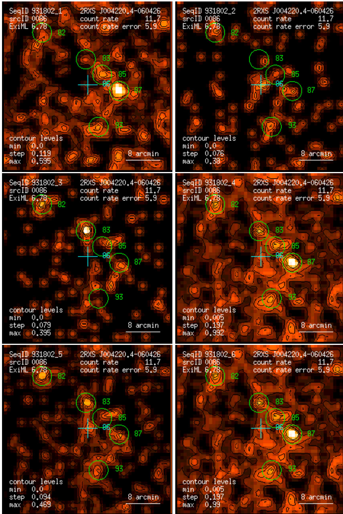
Figure 86: RASS 931802: detection 0086: band rate images, Gaussian filter: (1) PSPC channels 11 – 41, (2) 52 – 90, (3) 91 – 201, (4) 11 – 235, (5) 52 – 201, (6) 11 – 201. Broad band rates in counts/ks. Band rate contour levels in counts/ks/arcmin 2 .
