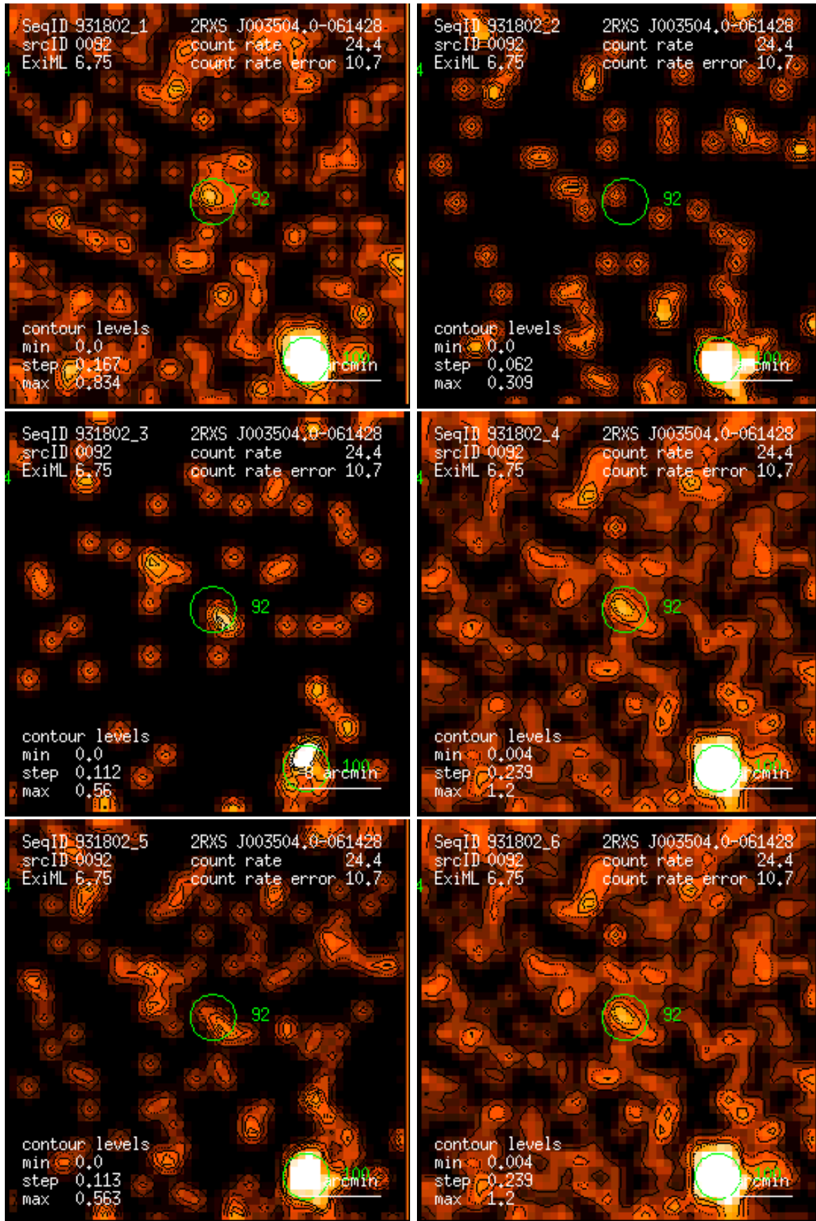
Figure 92: RASS 931802: detection 0092: band rate images, Gaussian filter: (1) PSPC channels 11 – 41, (2) 52 – 90, (3) 91 – 201, (4) 11 – 235, (5) 52 – 201, (6) 11 – 201. Broad band rates in counts/ks. Band rate contour levels in counts/ks/arcmin 2 .
