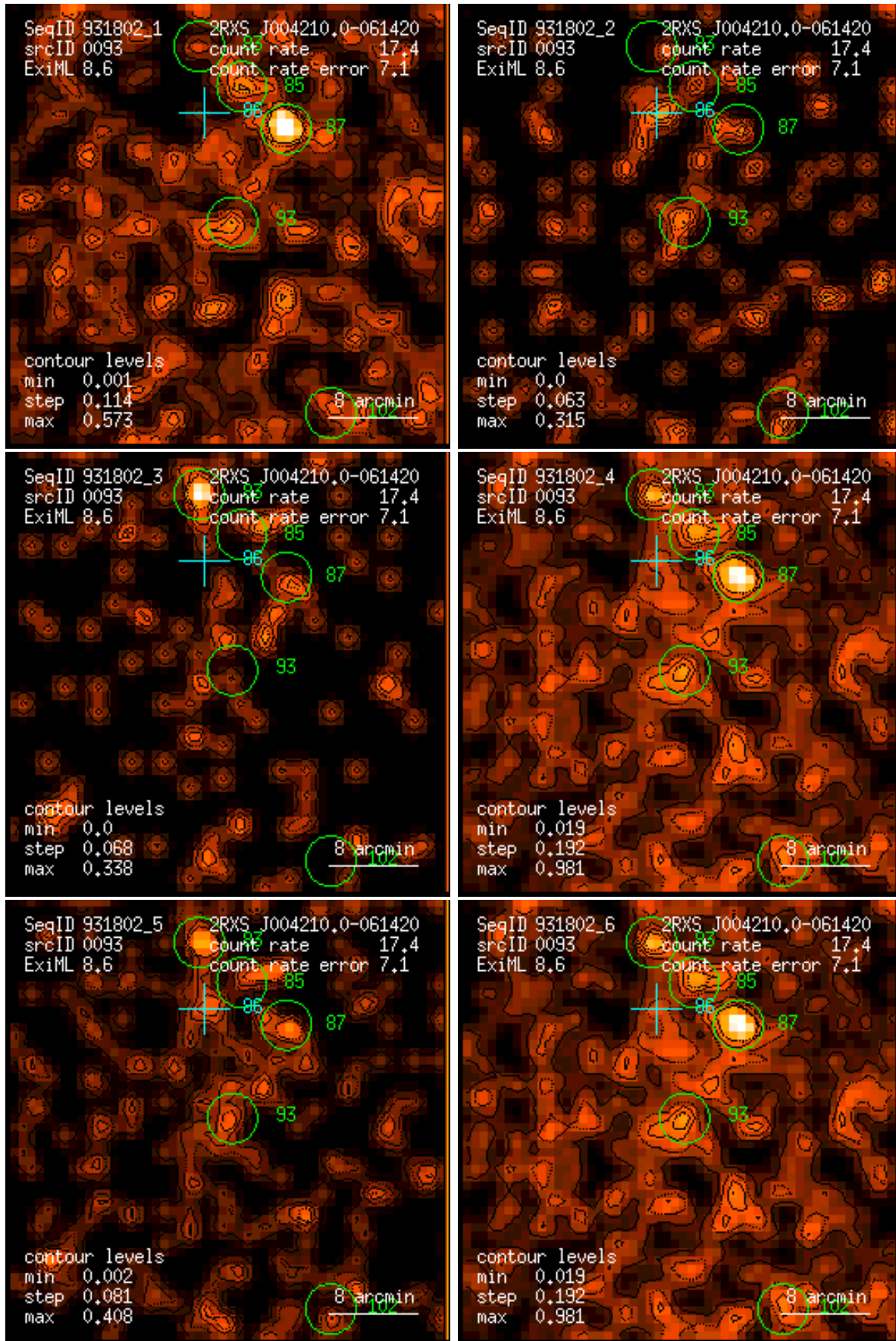
Figure 93: RASS 931802: detection 0093: band rate images, Gaussian filter: (1) PSPC channels 11 – 41, (2) 52 – 90, (3) 91 – 201, (4) 11 – 235, (5) 52 – 201, (6) 11 – 201. Broad band rates in counts/ks. Band rate contour levels in counts/ks/arcmin 2 .
