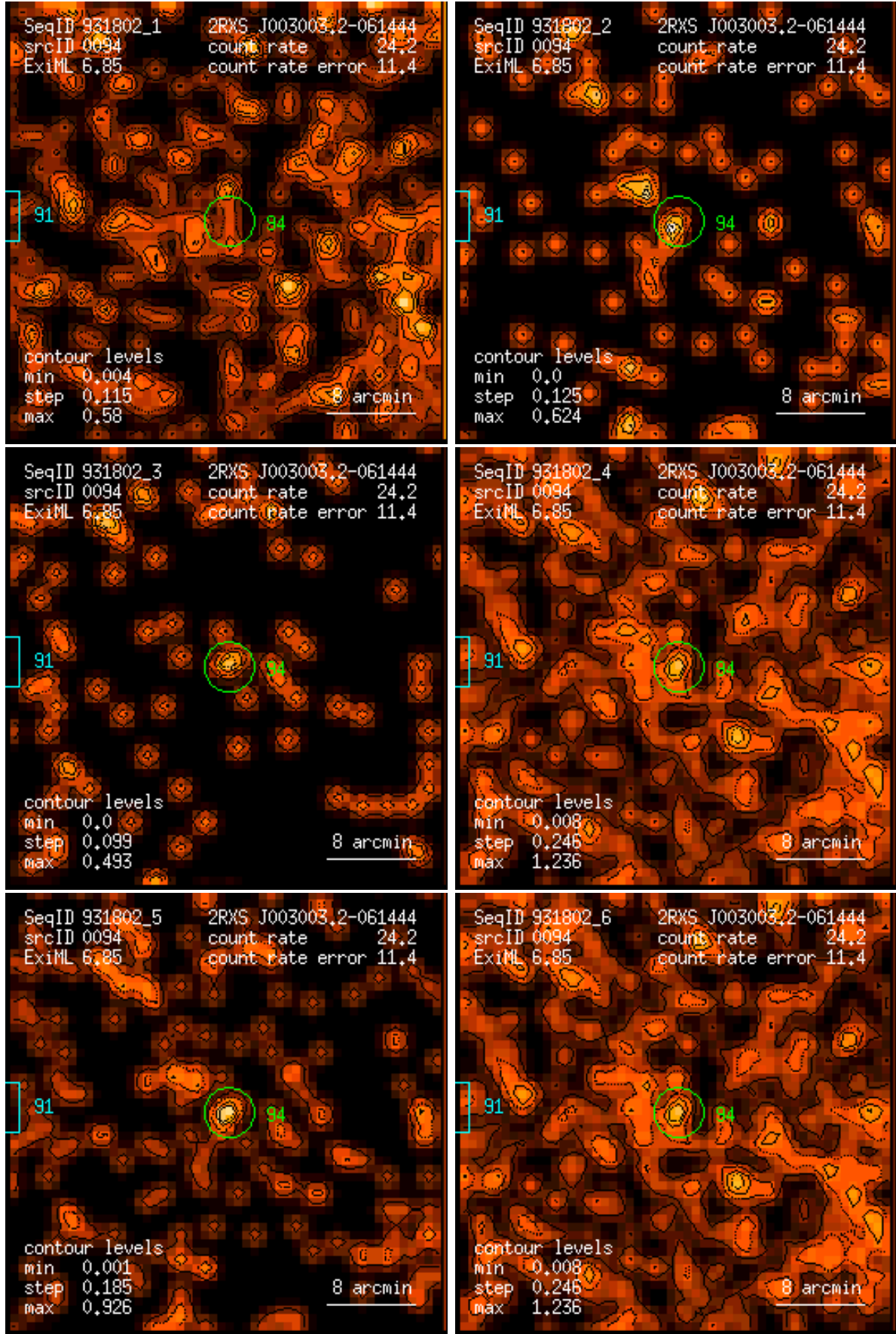
Figure 94: RASS 931802: detection 0094: band rate images, Gaussian filter: (1) PSPC channels 11 – 41, (2) 52 – 90, (3) 91 – 201, (4) 11 – 235, (5) 52 – 201, (6) 11 – 201. Broad band rates in counts/ks. Band rate contour levels in counts/ks/arcmin 2 .
