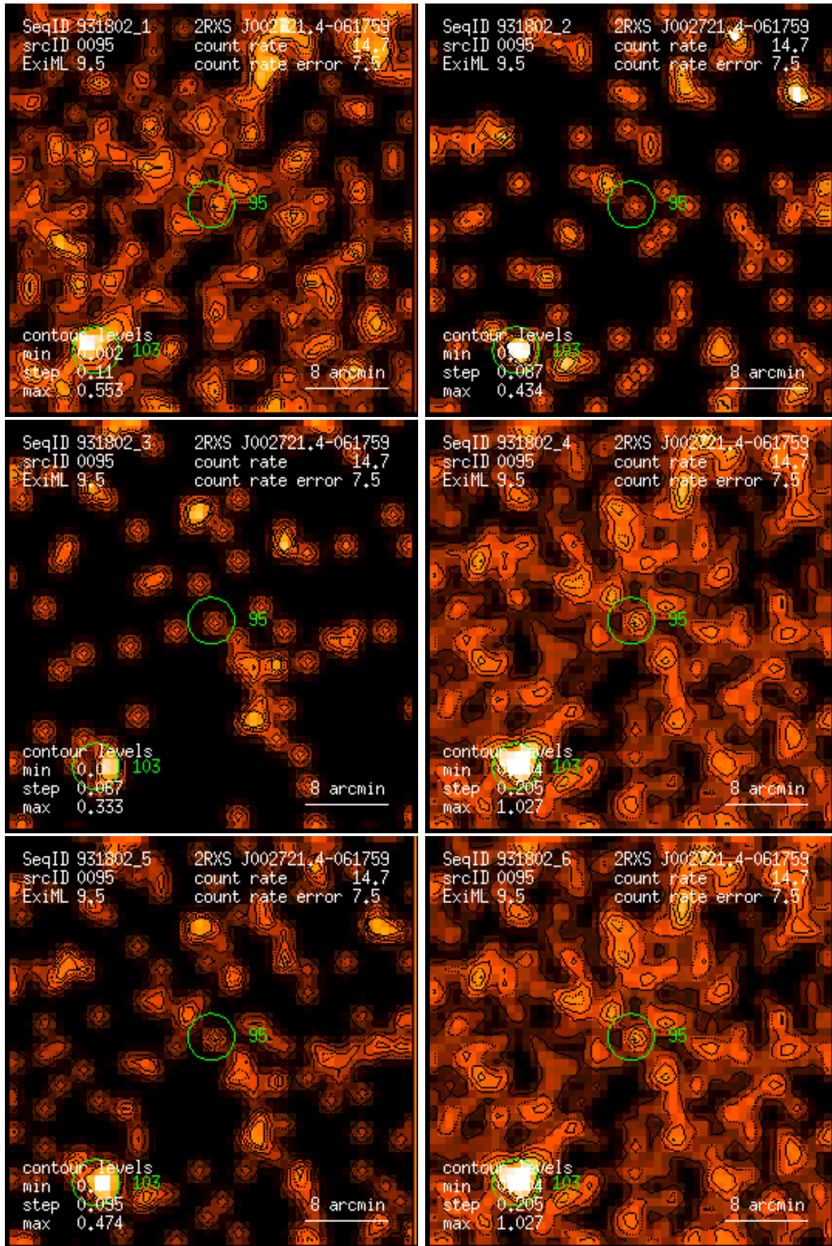
Figure 95: RASS 931802: detection 0095: band rate images, Gaussian filter: (1) PSPC channels 11 – 41, (2) 52 – 90, (3) 91 – 201, (4) 11 – 235, (5) 52 – 201, (6) 11 – 201. Broad band rates in counts/ks. Band rate contour levels in counts/ks/arcmin 2 .
