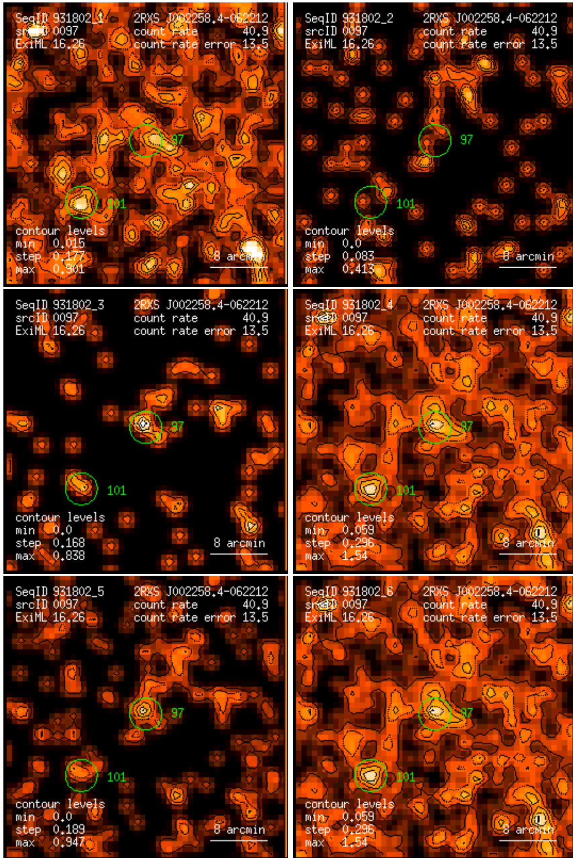
Figure 97: RASS 931802: detection 0097: band rate images, Gaussian filter: (1) PSPC channels 11 – 41, (2) 52 – 90, (3) 91 – 201, (4) 11 – 235, (5) 52 – 201, (6) 11 – 201. Broad band rates in counts/ks. Band rate contour levels in counts/ks/arcmin 2 .
