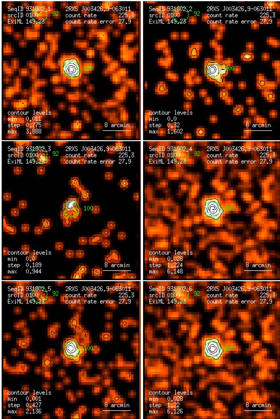
Figure 100: RASS 931802: detection 0100: band rate images, Gaussian filter: (1) PSPC channels 11 – 41, (2) 52 – 90, (3) 91 – 201, (4) 11 – 235, (5) 52 – 201, (6) 11 – 201. Broad band rates in counts/ks. Band rate contour levels in counts/ks/arcmin 2 .
