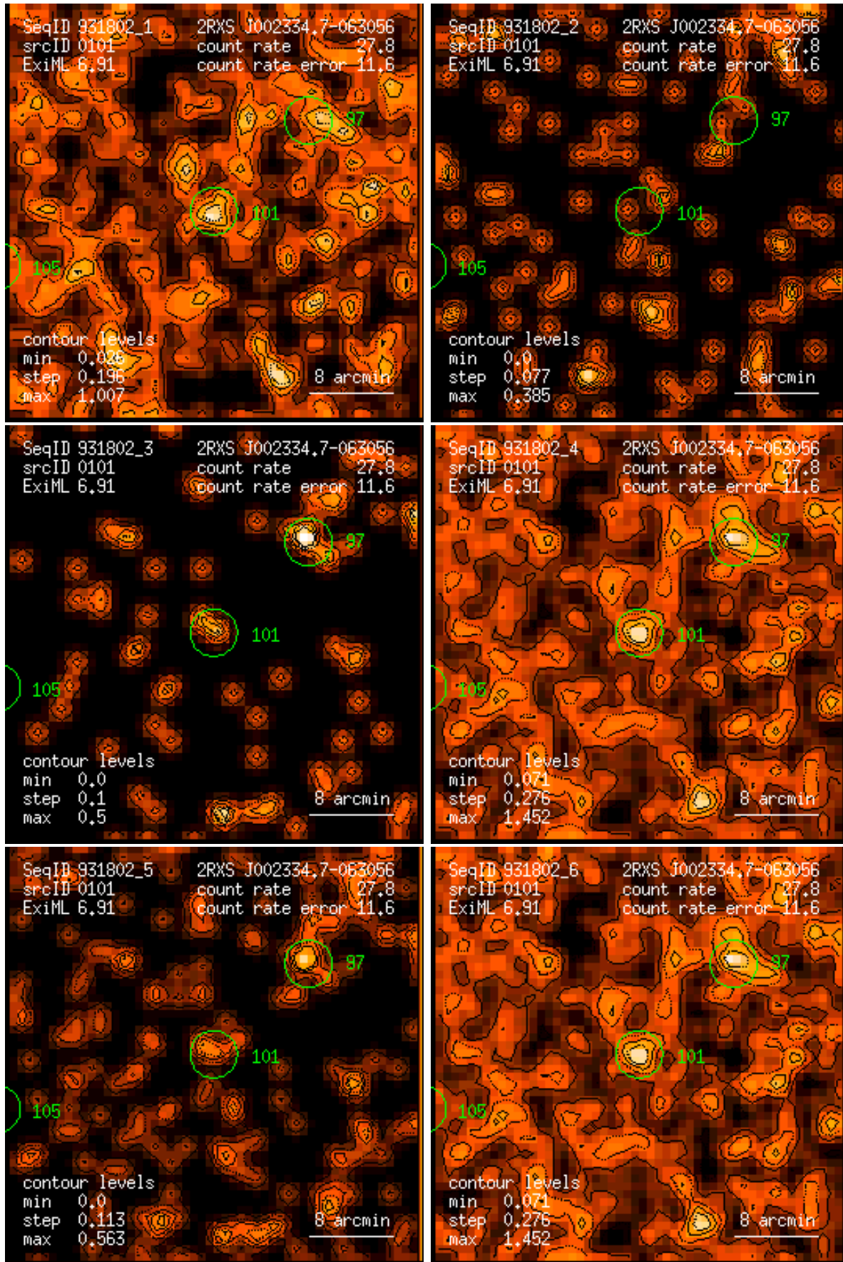
Figure 101: RASS 931802: detection 0101: band rate images, Gaussian filter: (1) PSPC channels 11 – 41, (2) 52 – 90, (3) 91 – 201, (4) 11 – 235, (5) 52 – 201, (6) 11 – 201. Broad band rates in counts/ks. Band rate contour levels in counts/ks/arcmin 2 .
