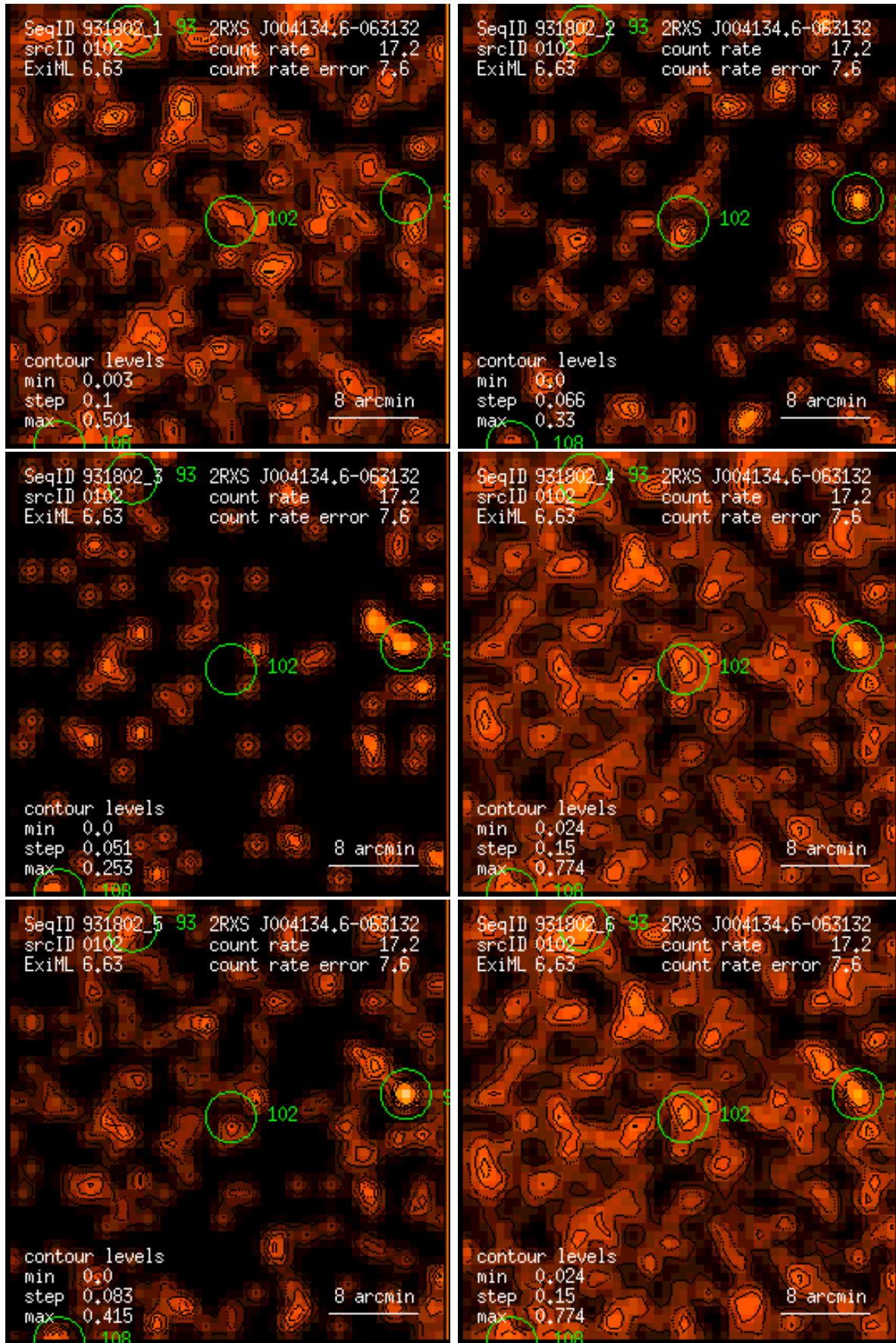
Figure 102: RASS 931802: detection 0102: band rate images, Gaussian filter: (1) PSPC channels 11 – 41, (2) 52 – 90, (3) 91 – 201, (4) 11 – 235, (5) 52 – 201, (6) 11 – 201. Broad band rates in counts/ks. Band rate contour levels in counts/ks/arcmin 2 .
